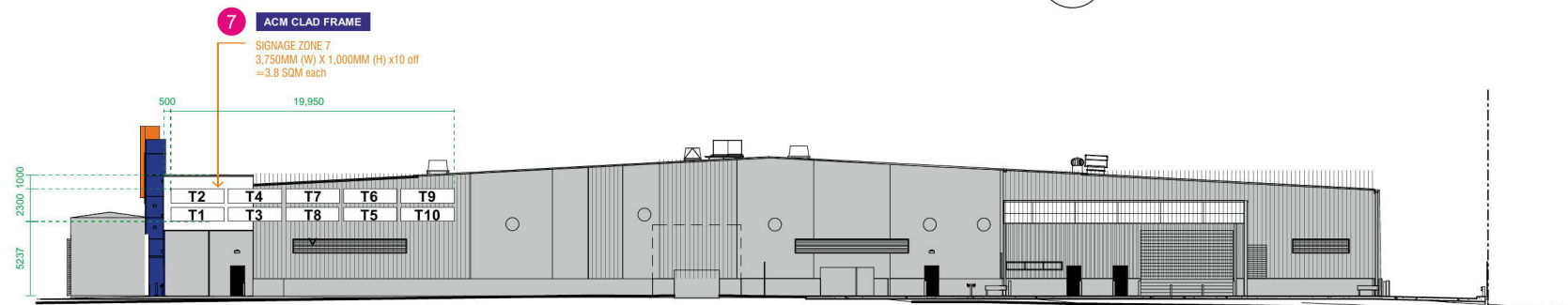
4 SOUTHEAST ELEVATION 20001
