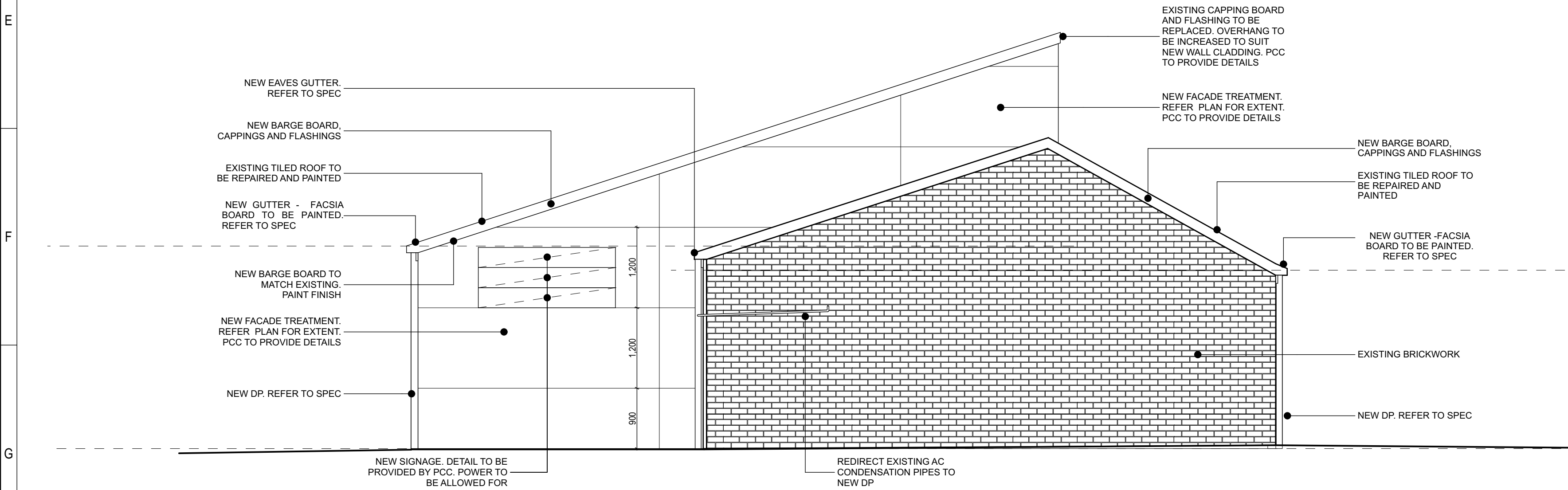
ELEVATION 04 SCALE 1:50
