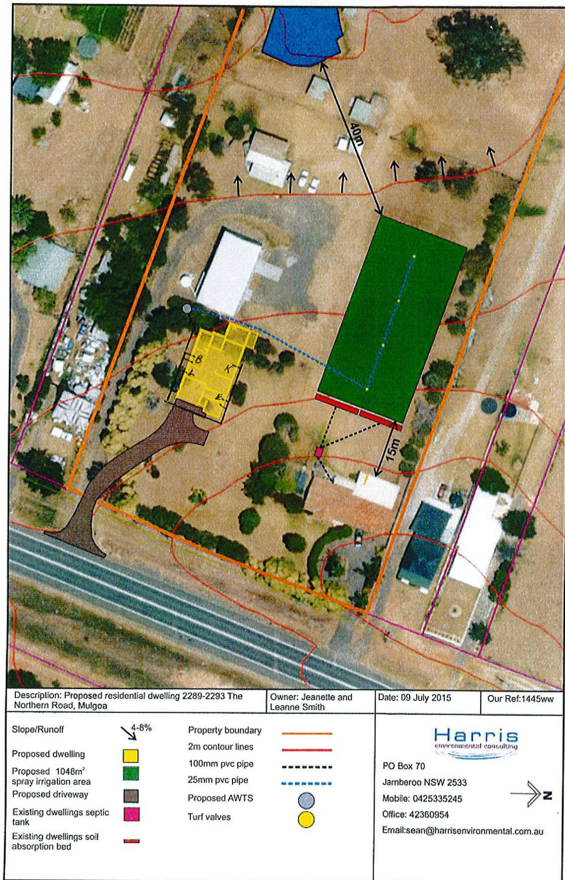
Figure 2 General Site Plan
