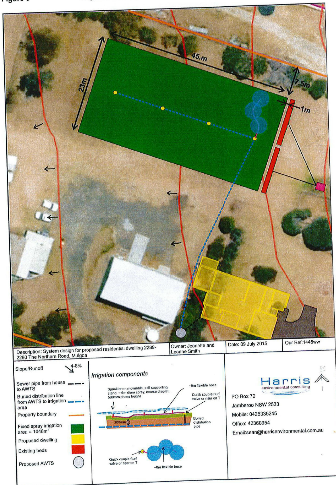
Figure 3 Irrigation Site Plan
