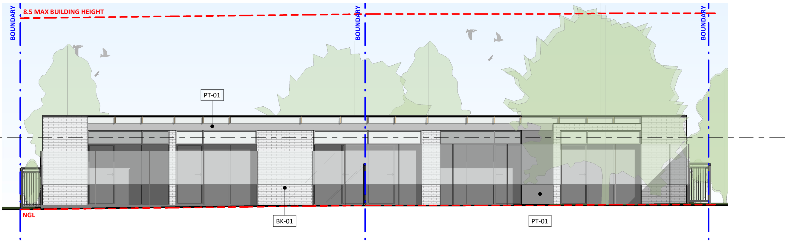
2 NORTHERN ELEVATION 1:100
