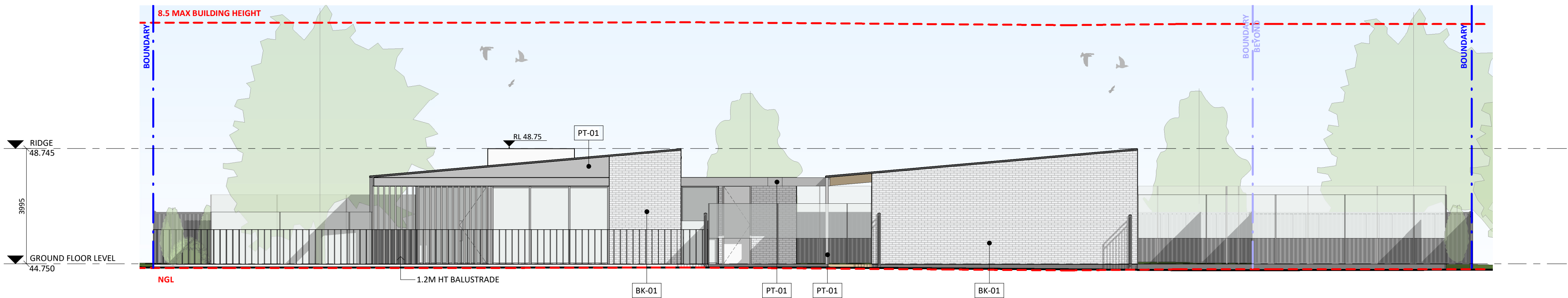
4 EASTERN ELEVATION 1:100
