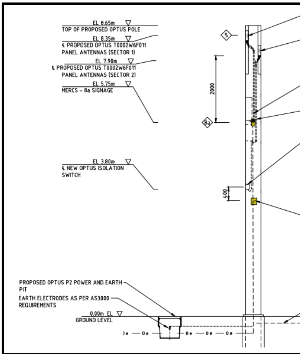
Figure 7: Smart Pole Equipment Layout.
