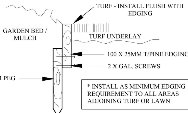
TYPICAL EDGING (NTS)
