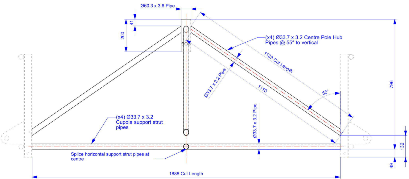
1054/1 Cupola Hub 1051/1 Quantity: (x1) off Material: 350 MPA Steel Pipe or as specified Finish: Black Paint Scale 1:10
