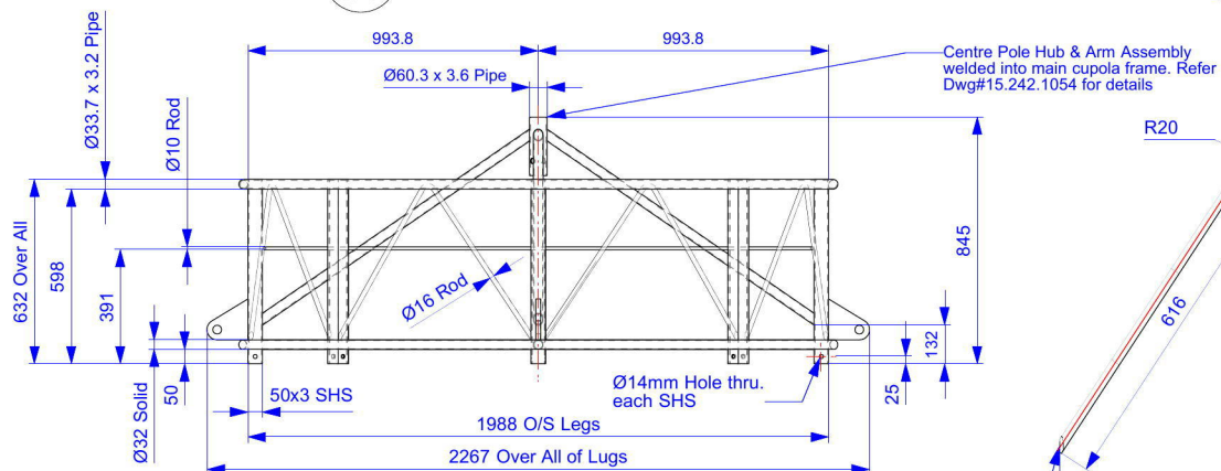
1051/1 Ø2m Cupola Ring Frame
