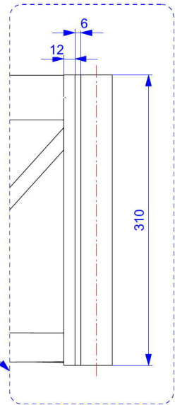
1033/3 Pin Detail Scale 1:10 Material: Grade 4140 round Qty: 2 Required per Bail Ring
