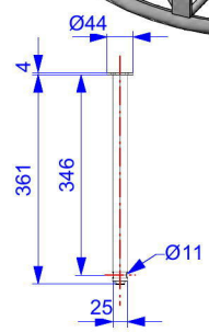
1033/3 Pin Detail Scale 1:10 Material: Grade 4140 round Qty: 2 Required per Bail Ring
