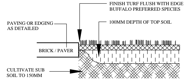
TURF PREPERATION DETAIL (NTS)
