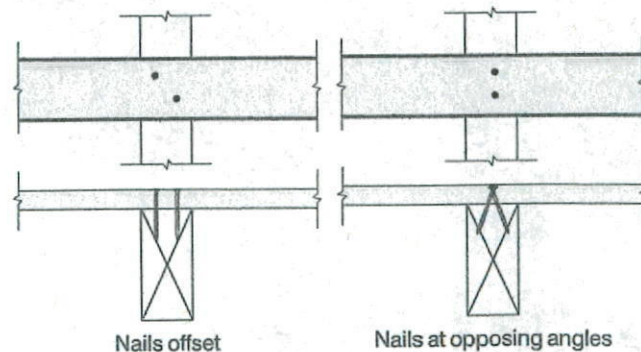
Nails offset
