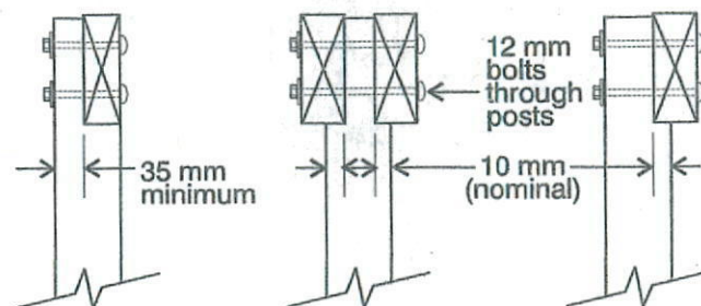
b) Bearers fully housed
