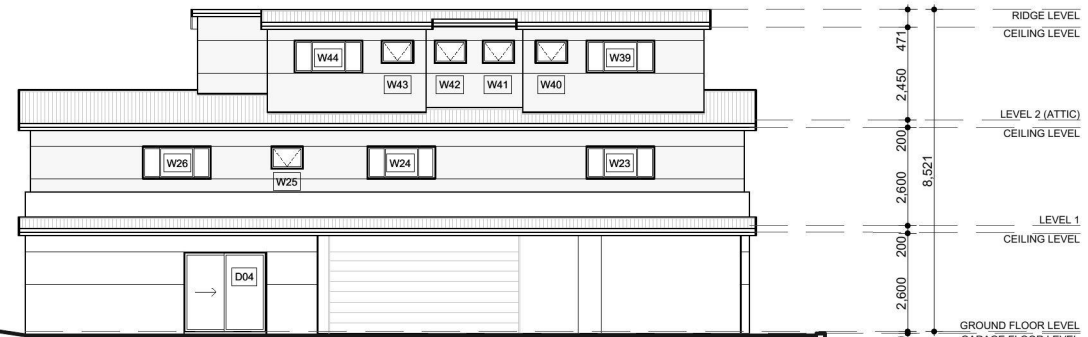
NORTH ELEVATION
