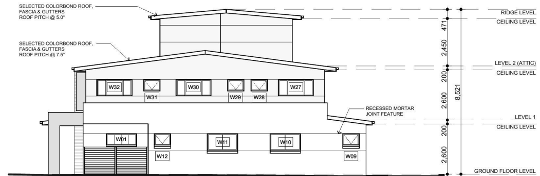
EAST ELEVATION
