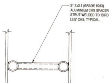
SECTION 5A SCALE 1:5
