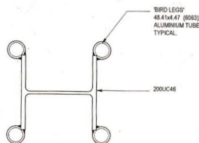
SECTION B SCALE 1:10
