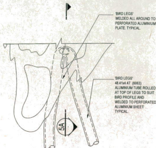
DETAIL 5 SCALE 1:10
