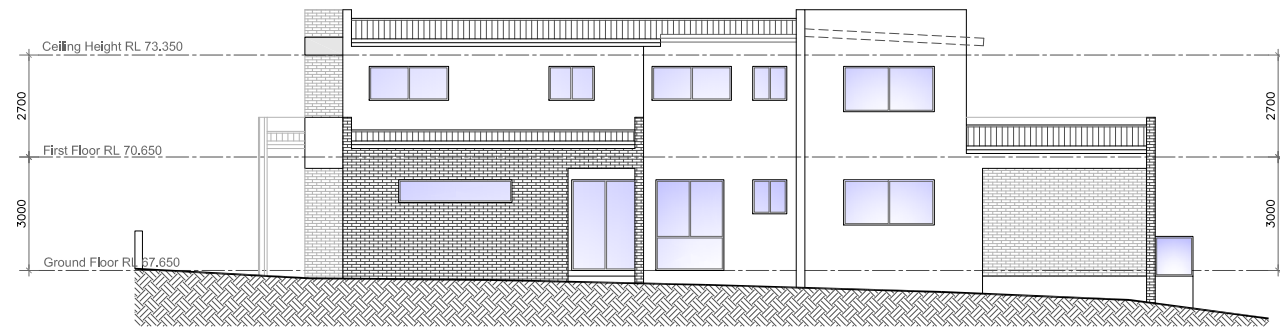
EAST ELEVATION
