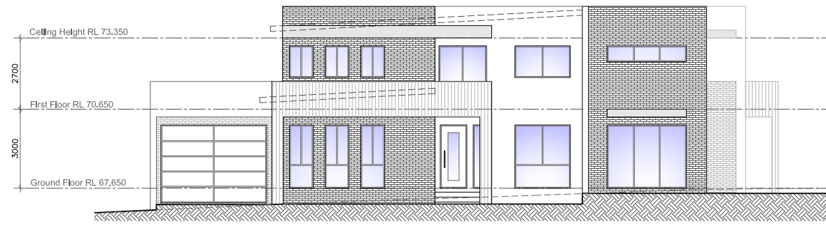
WEST ELEVATION
