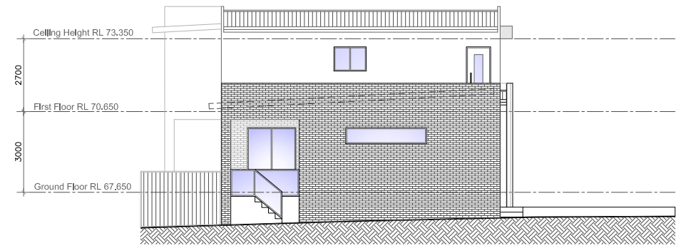
NORTH ELEVATION
