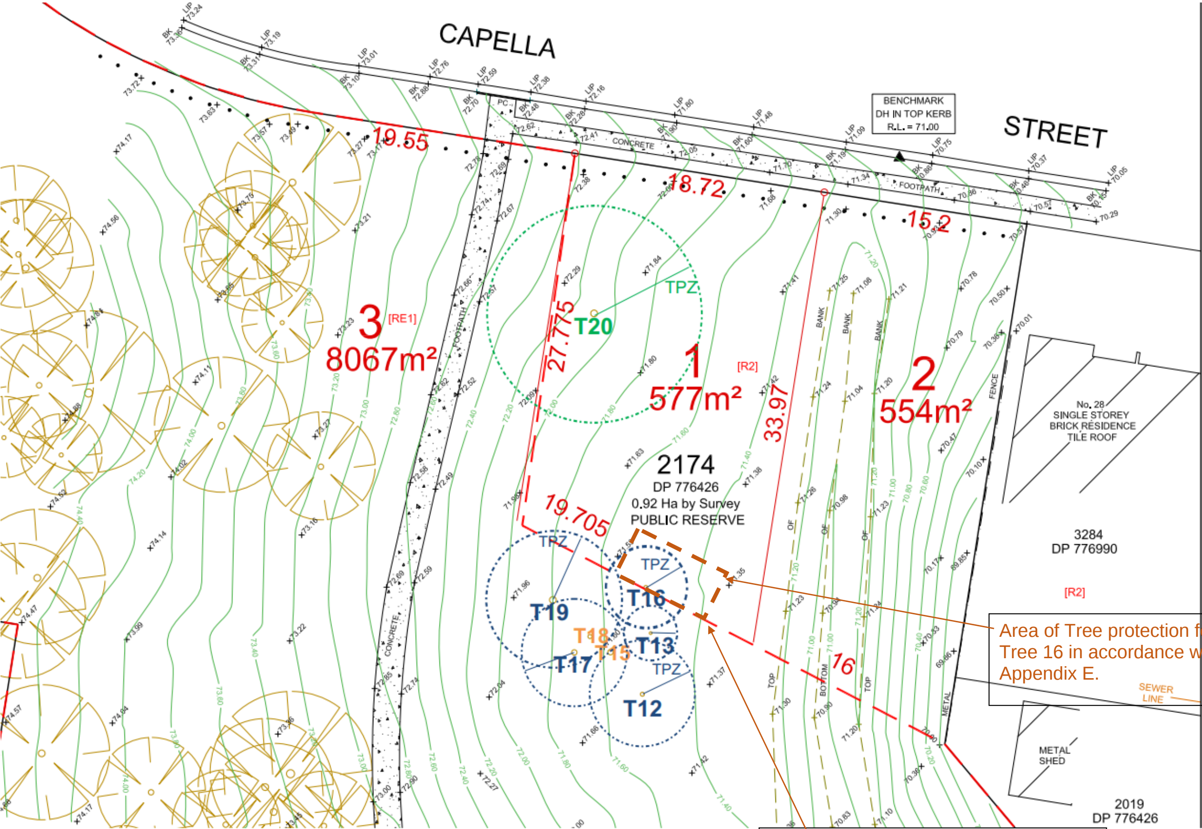
Plan of Detail and Levels dated 28/7/20 Version A by Richard Hogan and Company
