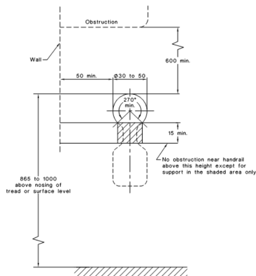
FIGURE 29 (in part) HANDRAILS
