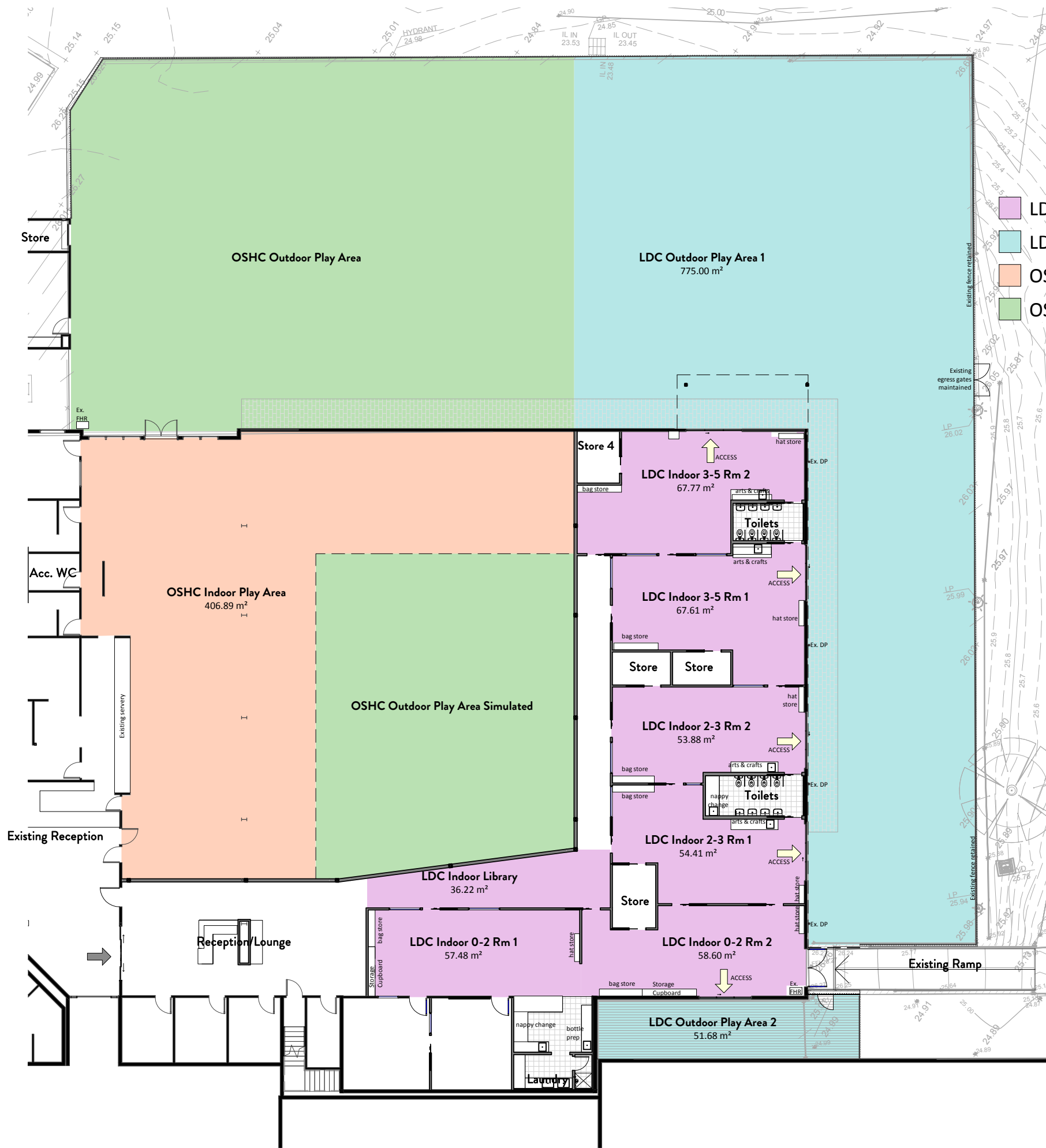
1 Ground Floor Plan - Areas 1 : 250
