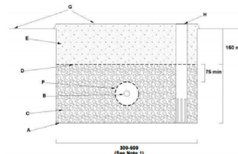
Cross Section: Pressure-dosed Trench
