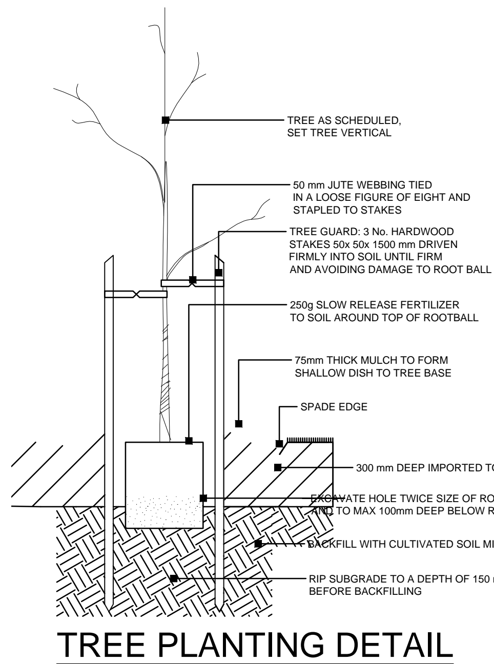
TREE PLANTING DETAIL
