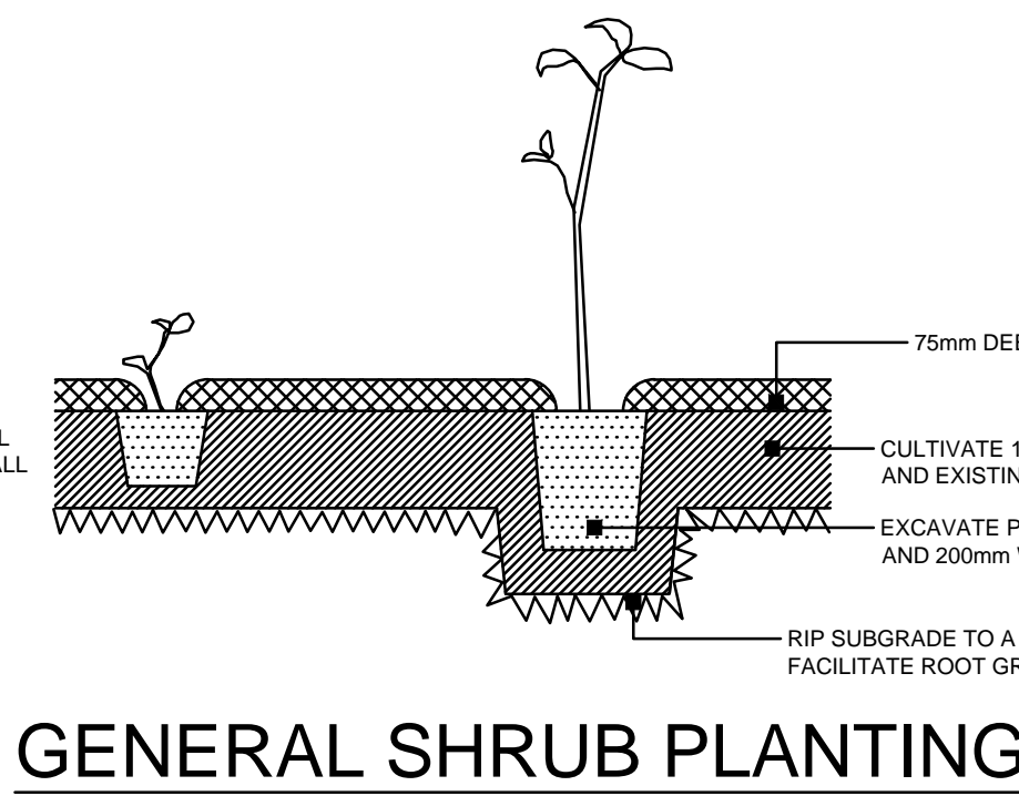
GENERAL SHRUB PLANTING
