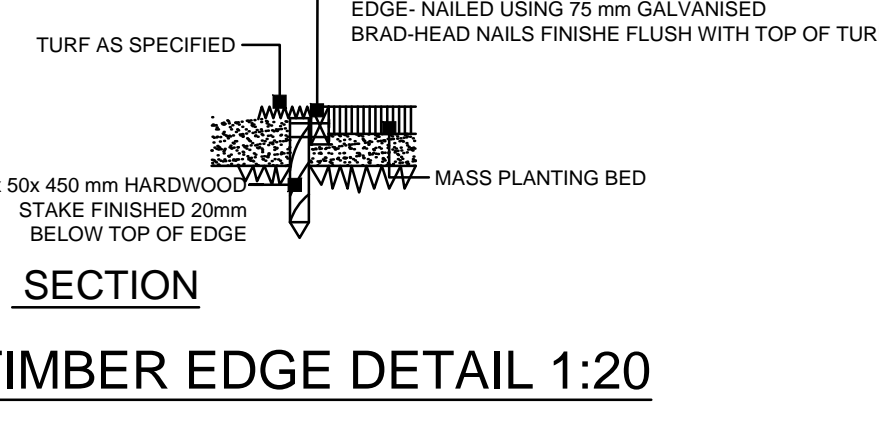
SECTION TIMBER EDGE DETAIL 1:20
