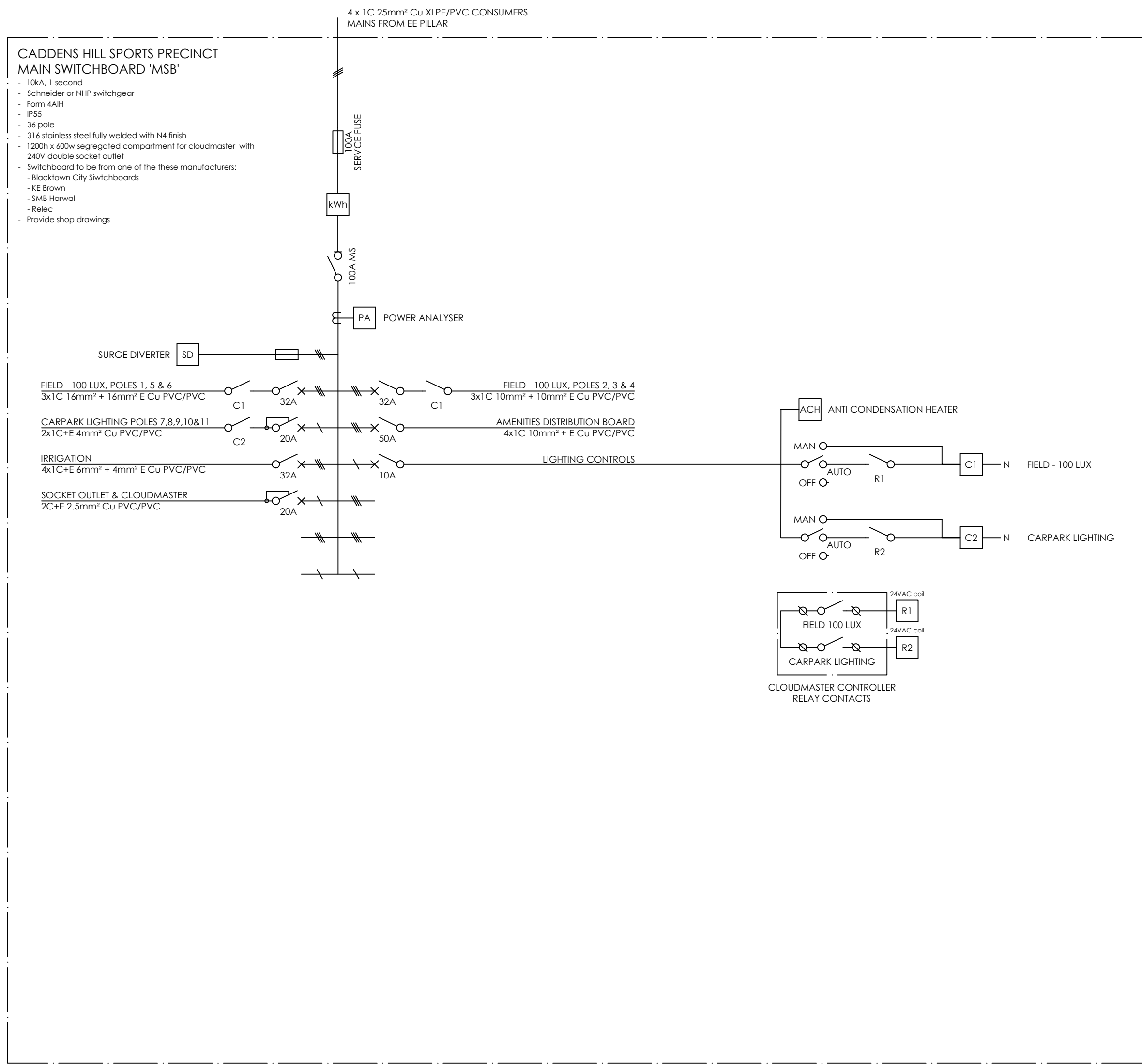
SINGLE LINE DIAGRAM
