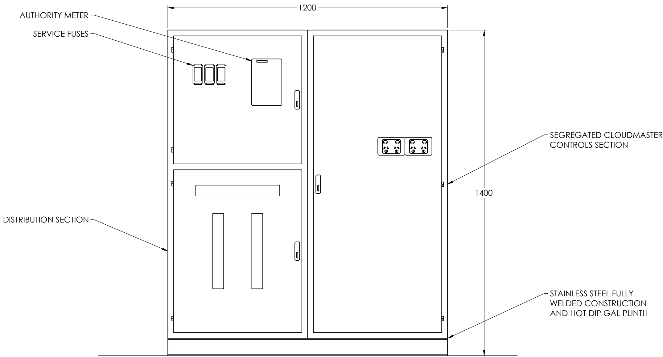
MAIN SWITCHBOARD ELEVATION
