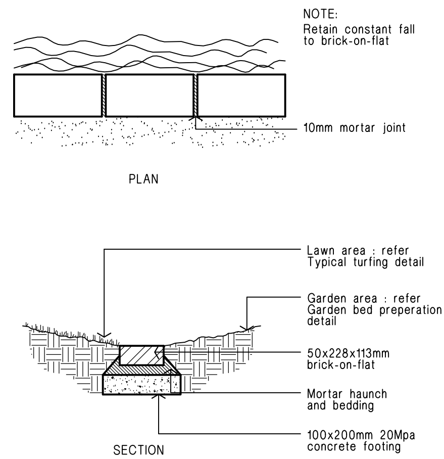
Brick garden edge Detail.
