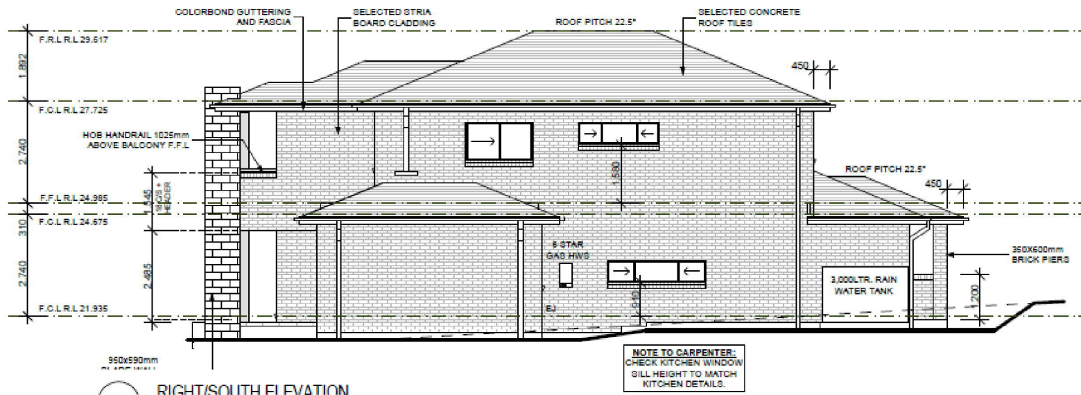
RIGHT/SOUTH ELEVATION
