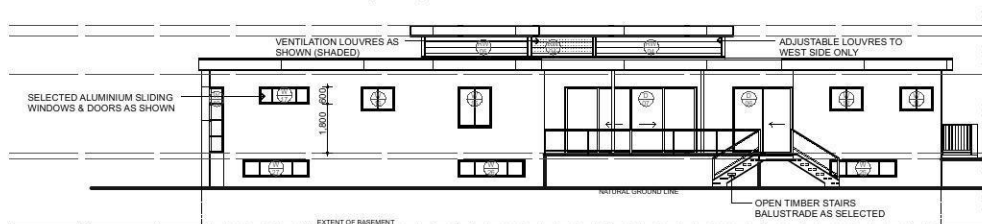
WEST ELEVATION
