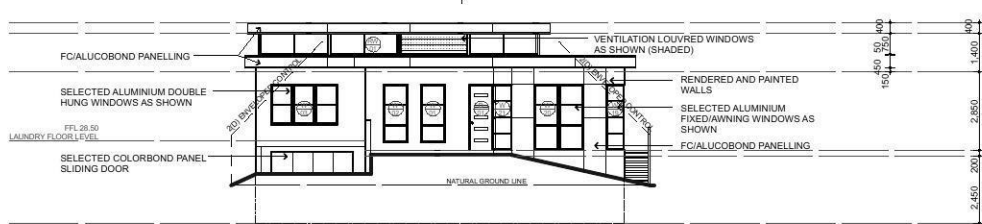
RODLEY AVENUE (NORTH) ELEVATION
