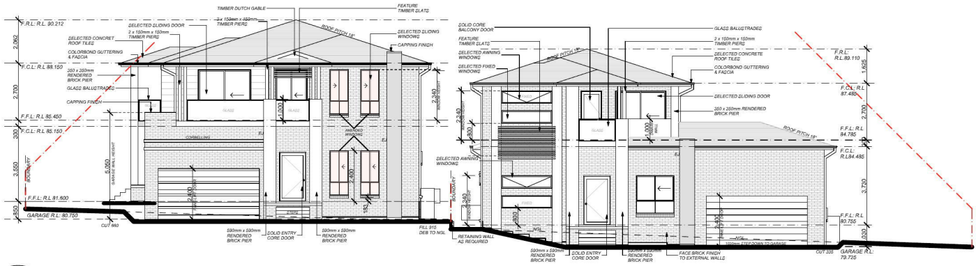
FRONT/NORTH ELEVATION 1:250
