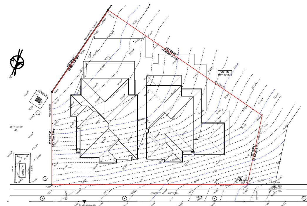
MACADAMIA COURT SHADOW PROJECTIONS 21ST JUNE 12PM 1:491.3181
