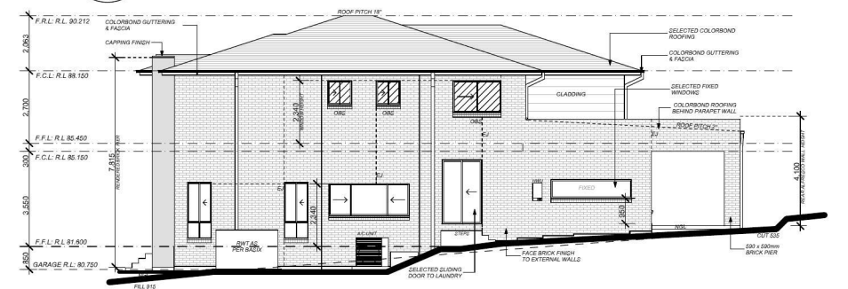
RIGHT/WEST ELEVATION 2 1:250
