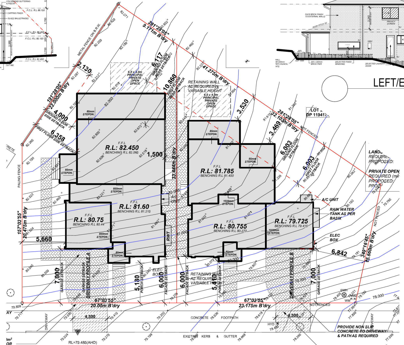
MACADAMIA COURT SITE PLAN 1:300
