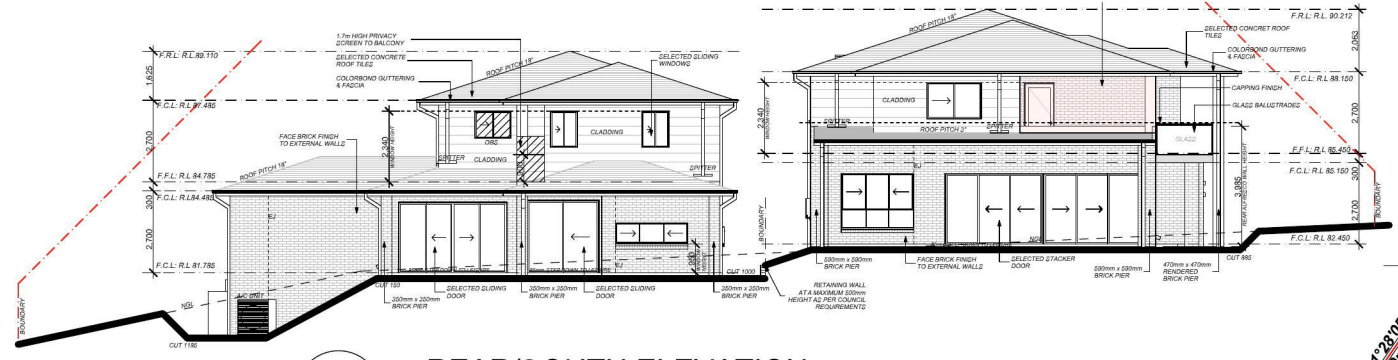
REAR/SOUTH ELEVATION 1:250
