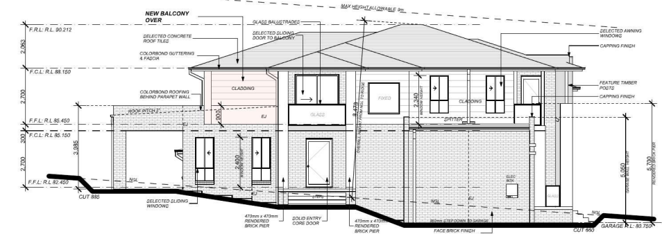
LEFT/EAST ELEVATION 1:250
