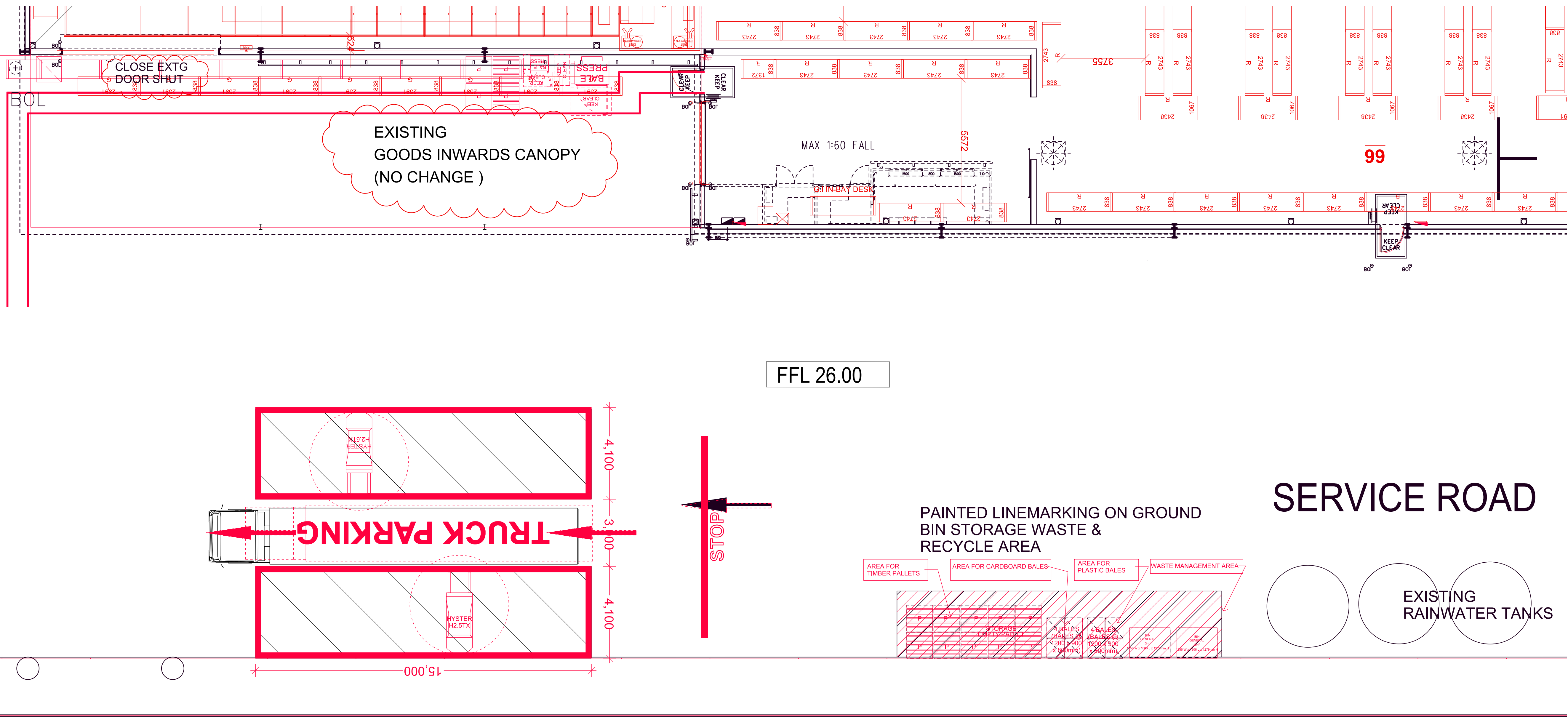
01 DETAIL - WASTE RECYCLE / SOUTH WEST END
