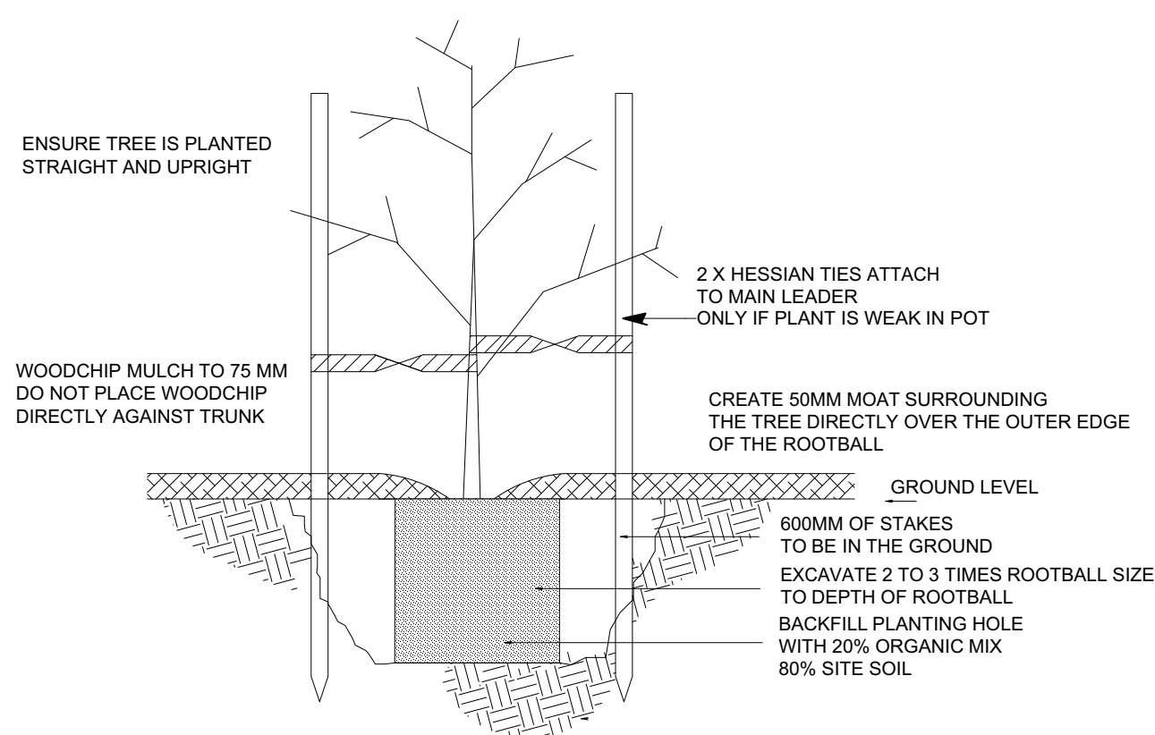
TREE PLANTING SCALE 1:10
