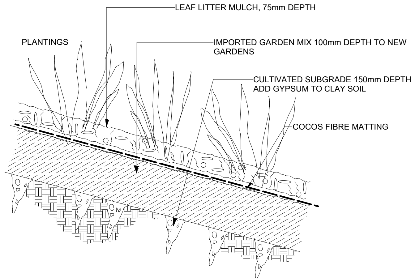
PLANTING EXCEEDING 1 : 4 SCALE 1:10
