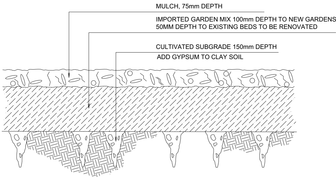
GARDEN BEDS ON GRADE SCALE 1:10
