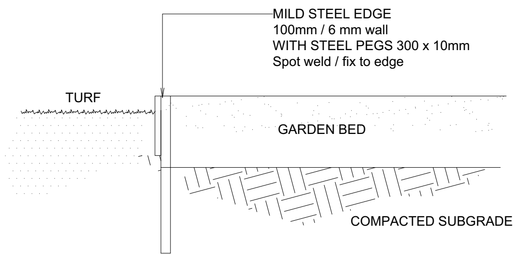
STEEL EDGING BETWEEN GARDENS AND TURF SCALE 1:10
