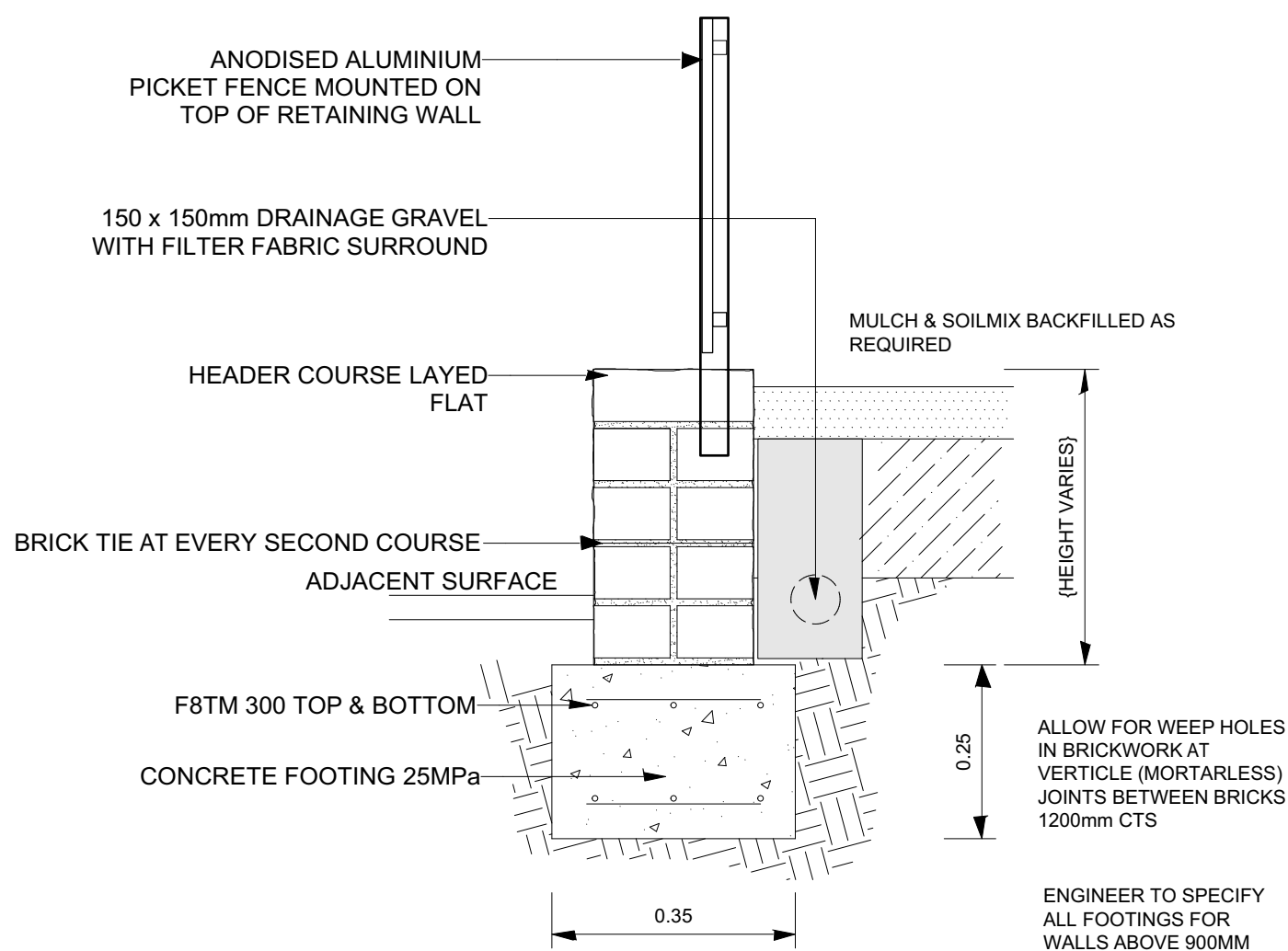
BRICK RETAINING WALL WITH FENCING MOUNTED SCALE 1:10
