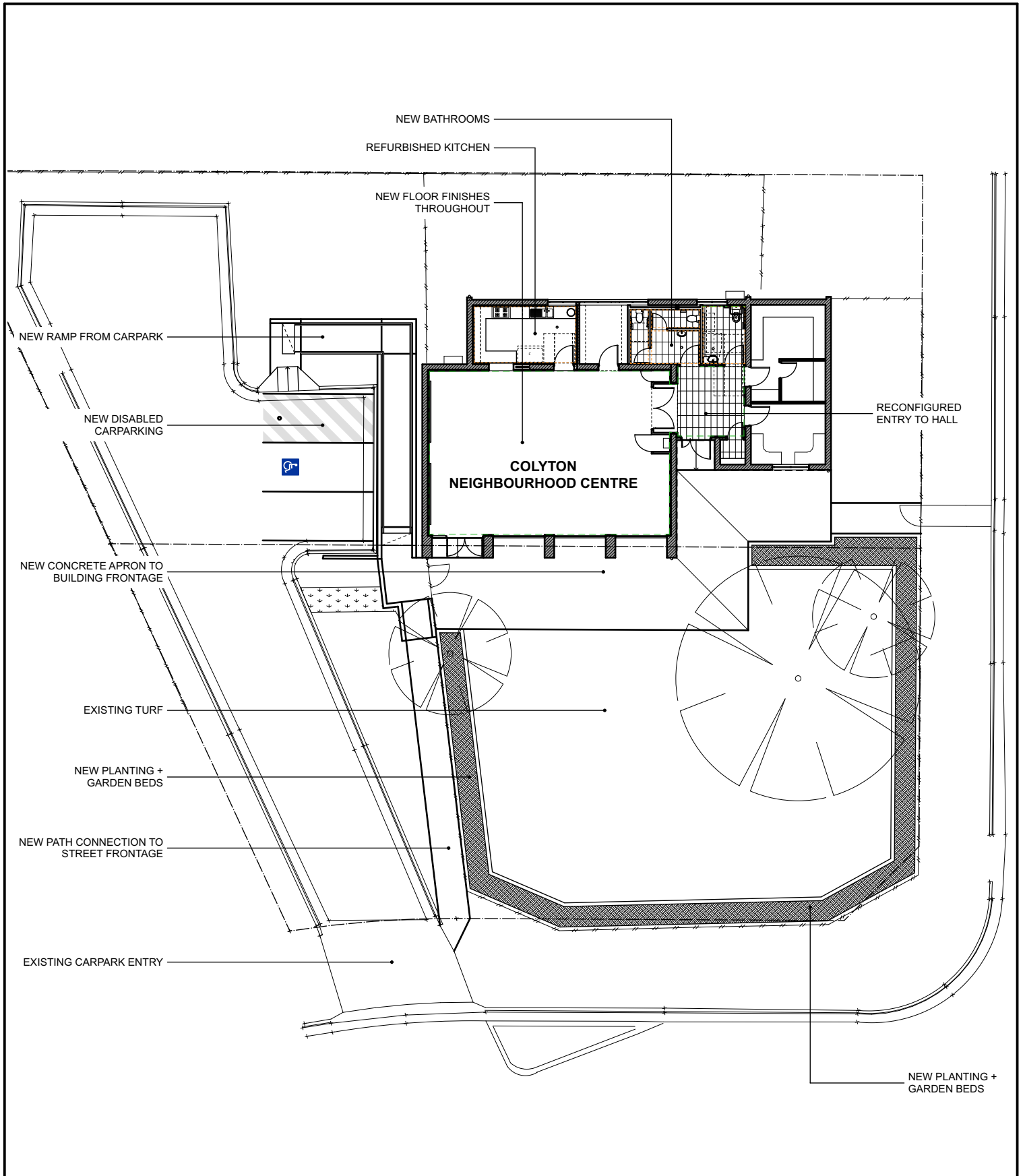
PROPOSED FLOOR PLAN SCALE 1:250
