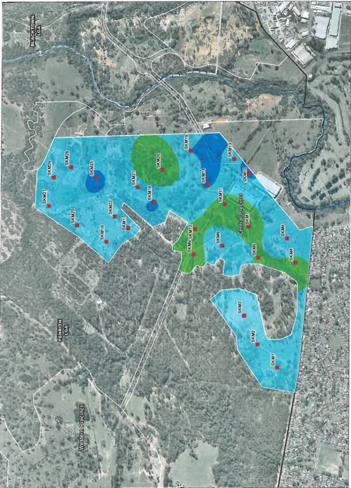
Fig 5.6 : Soil Salinity at a Depth of 0.5m (B-Horizon)
