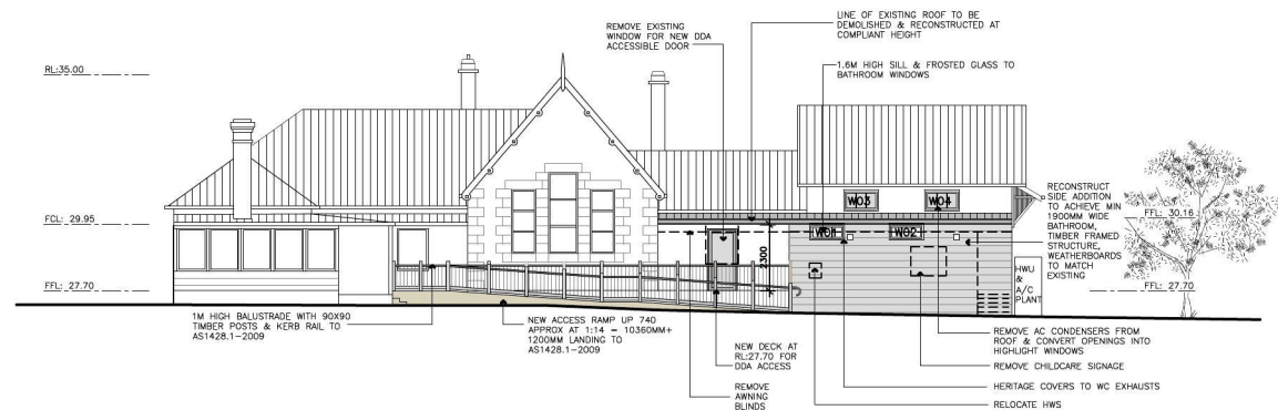
PROPOSED NORTHERN ELEVATION
