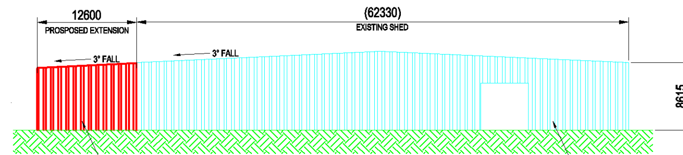
WEST ELEVATION
