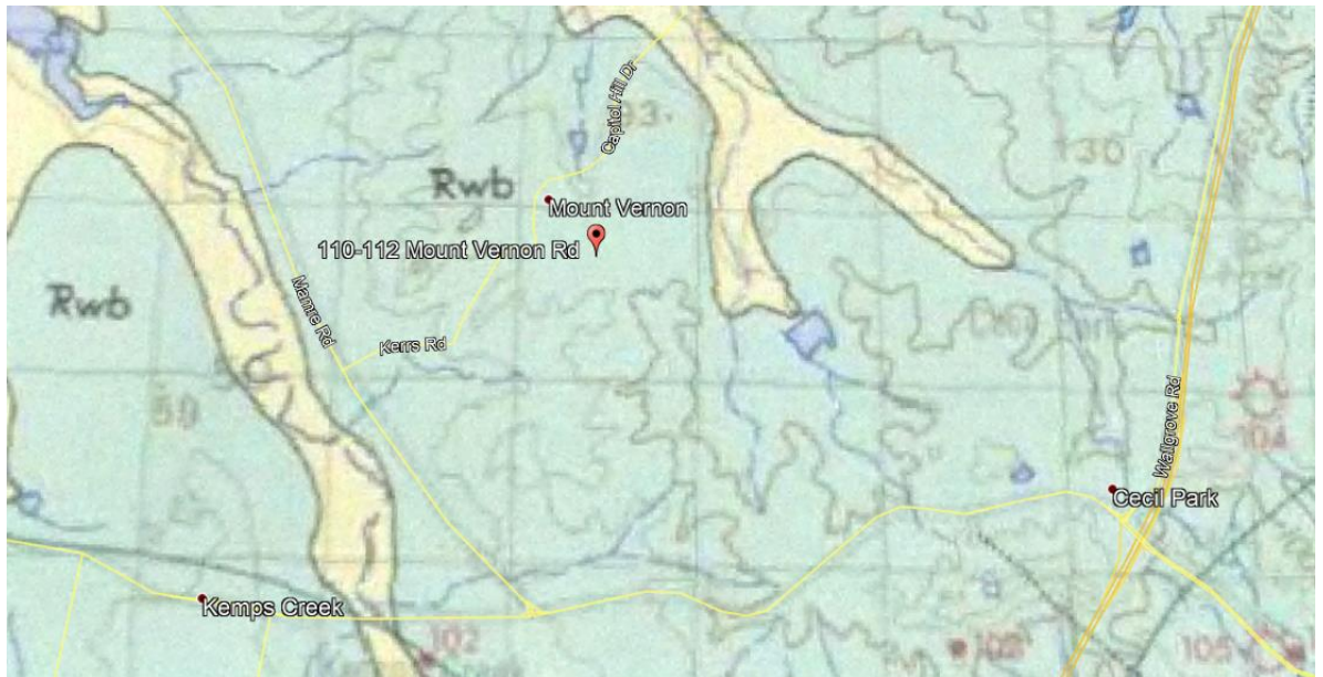
Figure 1 Geology Map Excerpt
