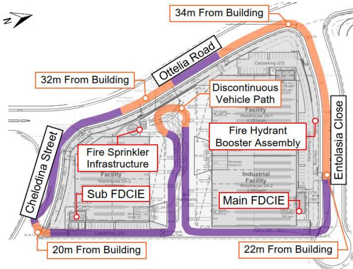
Figure 6-5: Vehicular Perimeter Path
