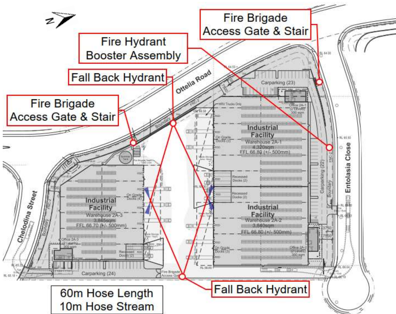
Figure 6-4: Fire Hydrant Infrastructure
