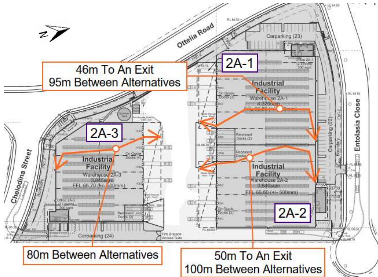
Figure 6-1: Speculative Non-Compliant Travel Distances Based On Standard Racking
