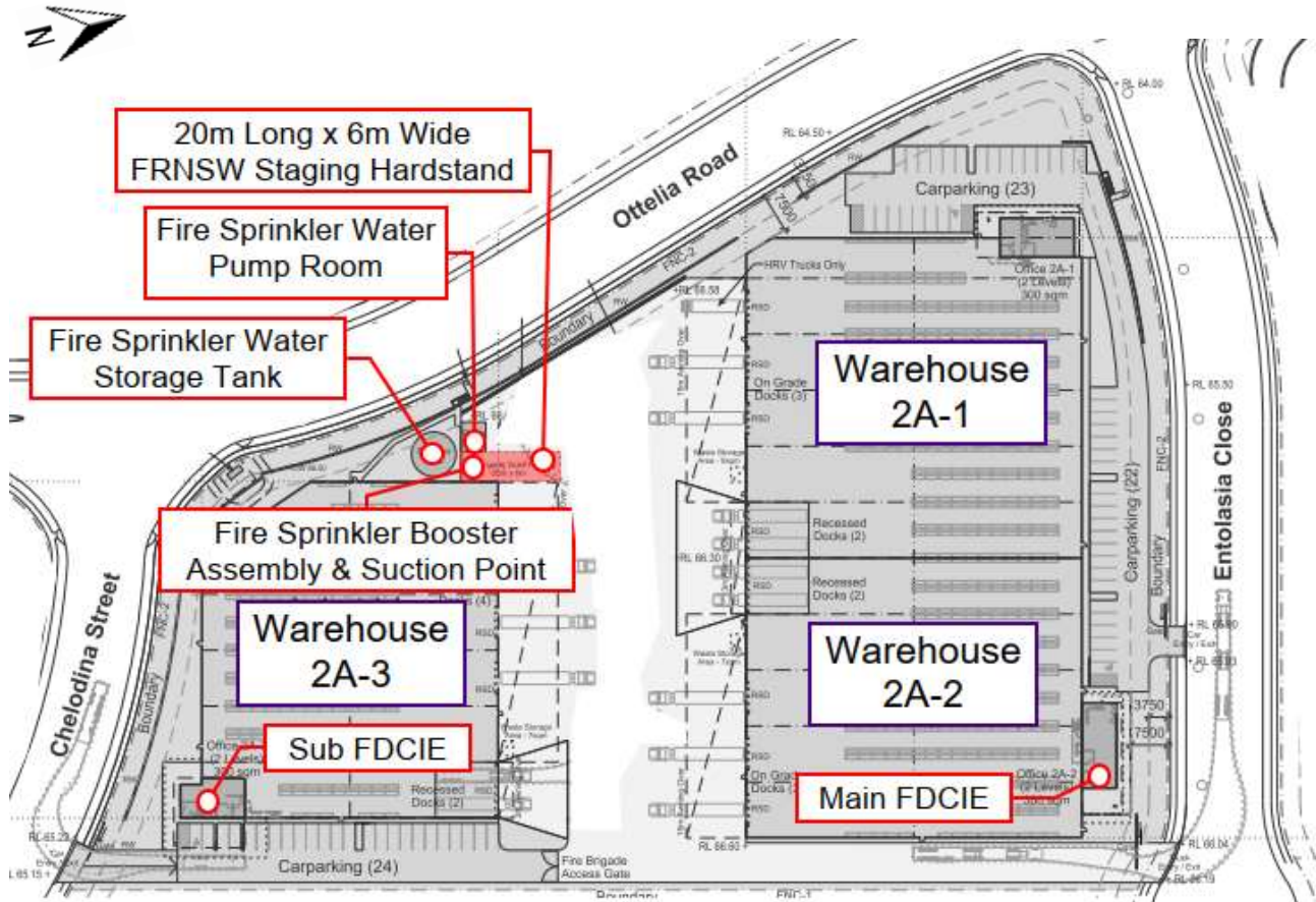
Figure 6-2: Fire Sprinkler Infrastructure & FDCIE Locations
