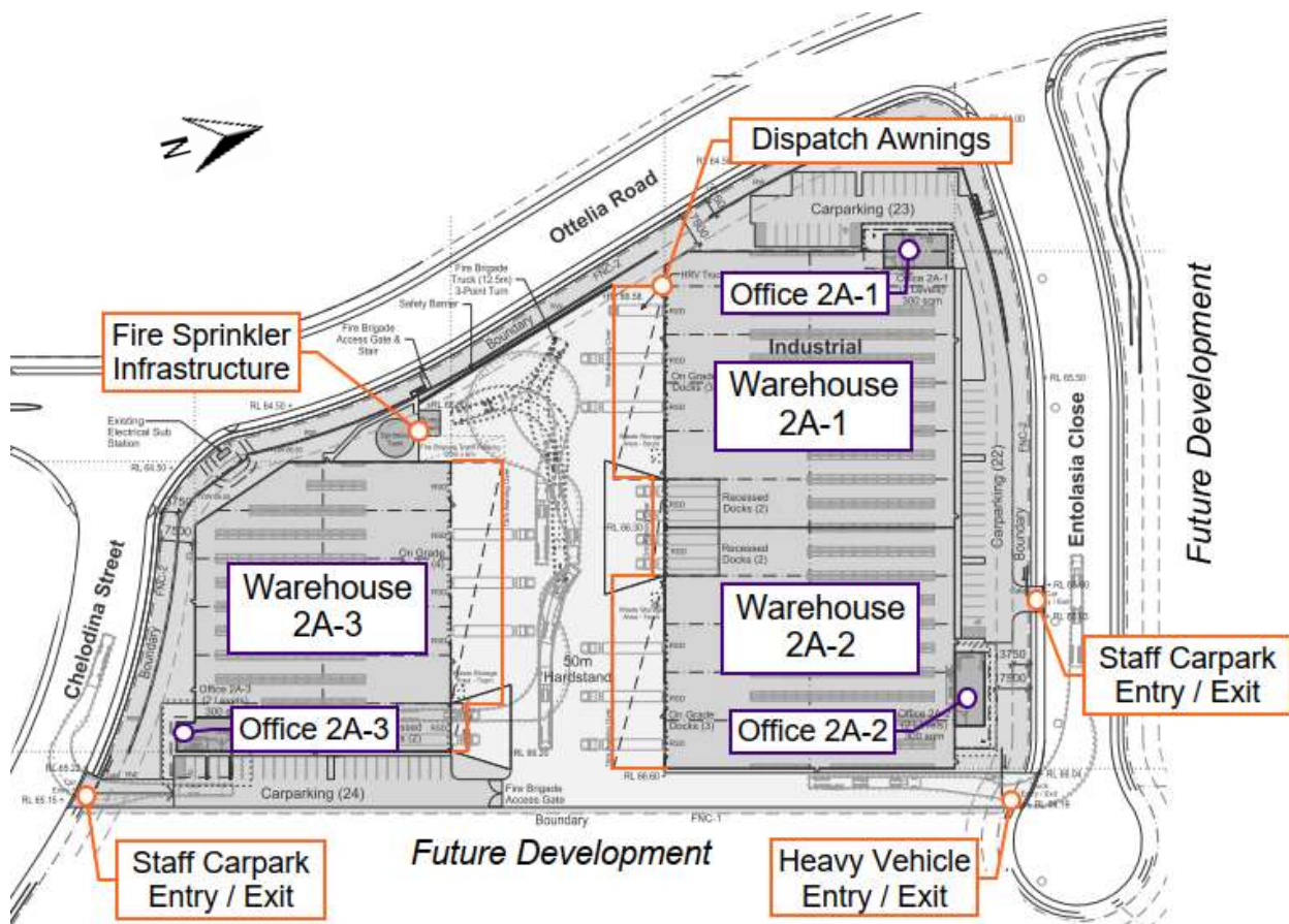
Figure 2-2: Site Plan Description
