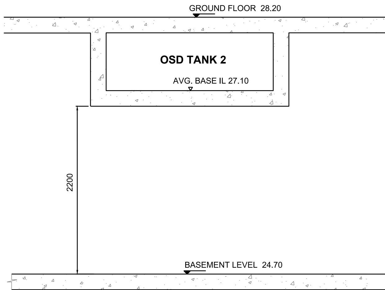
OSD 2 SECTION CLEARANCE TO BASEMENT FLOOR LEVEL NOT TO SCALE
