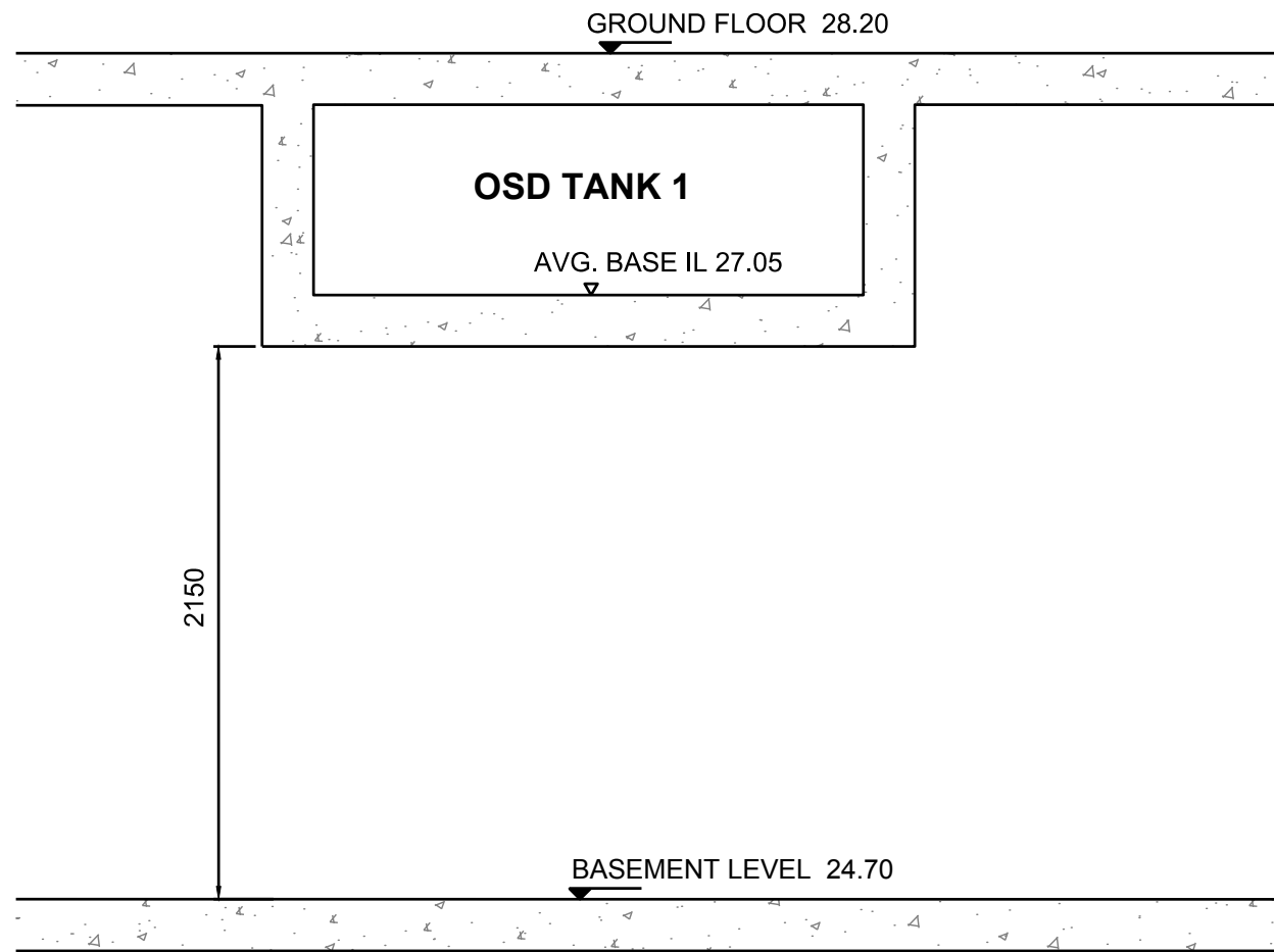
OSD 1 SECTION CLEARANCE TO BASEMENT FLOOR LEVEL NOT TO SCALE
