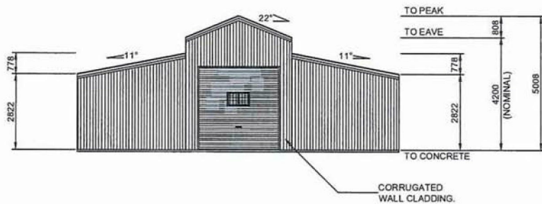
4 ENDWALL EXTERIOR ELEVATION
