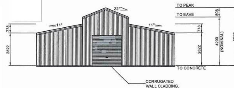
3 ENDWALL EXTERIOR ELEVATION
