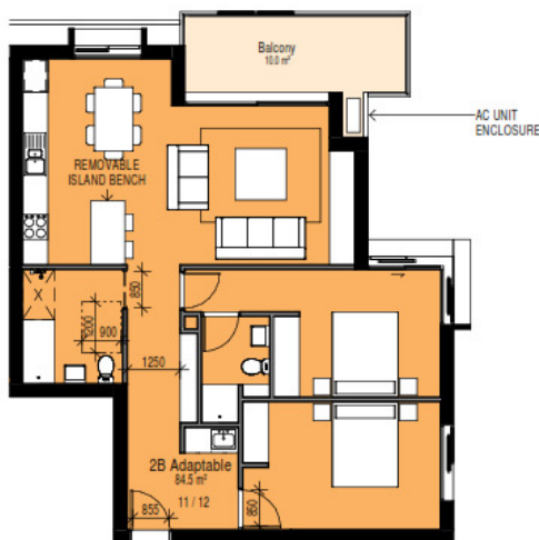
PRE-ADAPTABLE UNITS 11/12 AND LIVABLE
