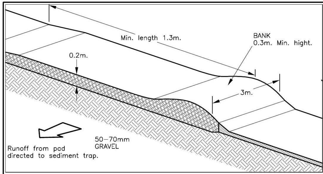
TEMPORARY CONSTRUCTION EXIT
