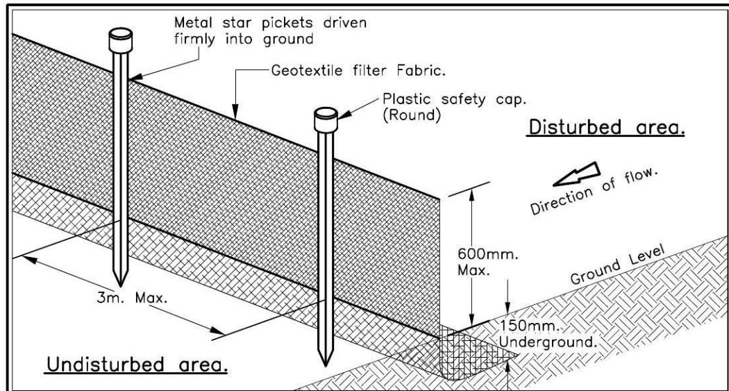
SEDIMENT FENCE
