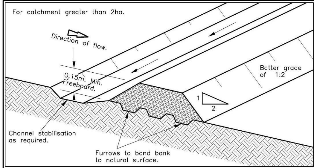
DIVERSION BANK AND CHANNEL
