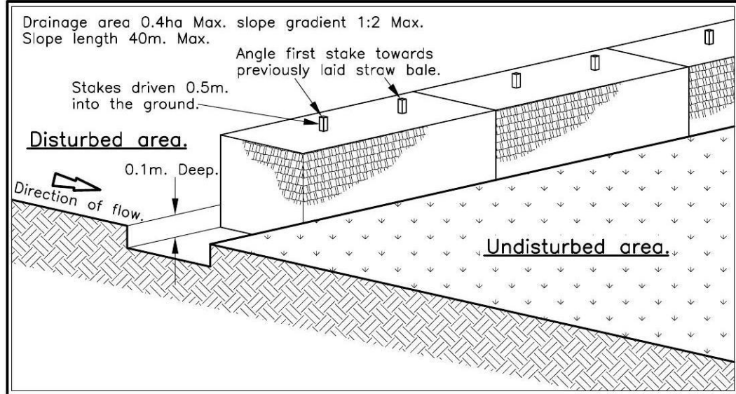
STRAW BALE SEDIMENT FILTER
