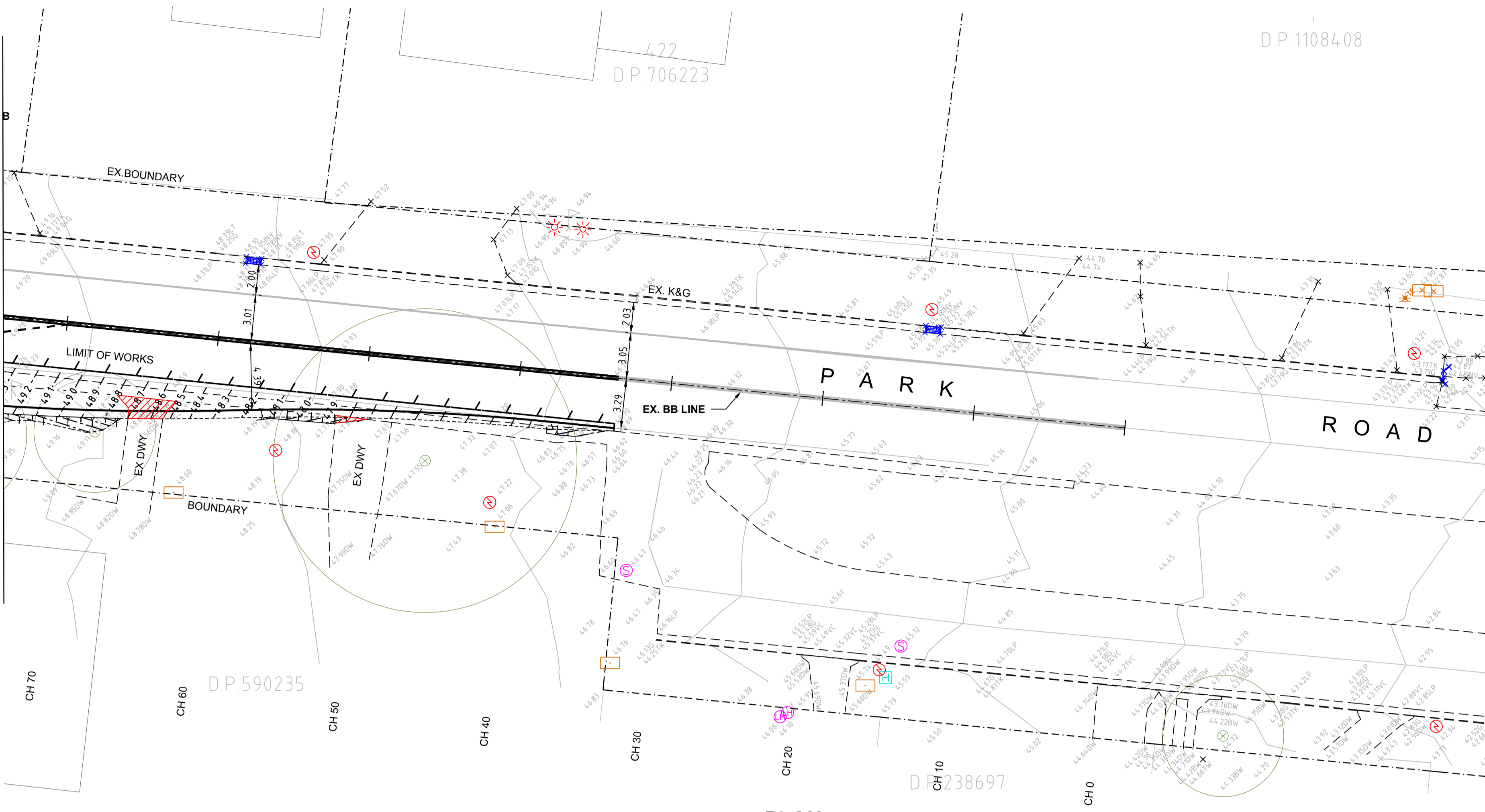
PLAN SCALE 1:200
