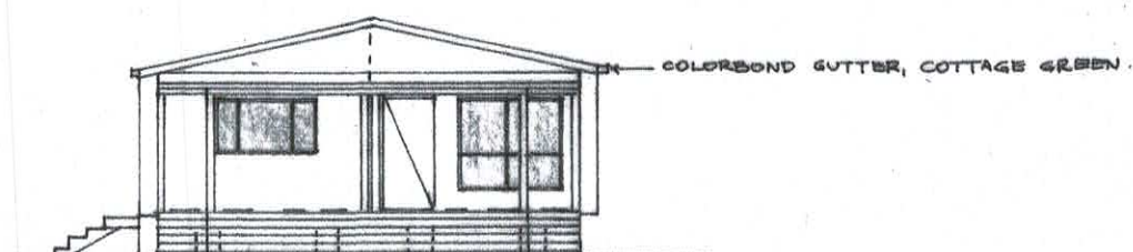
EAST ELEVATION 1:100
