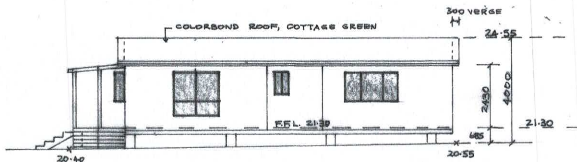
NORTH ELEVATION 1:100
