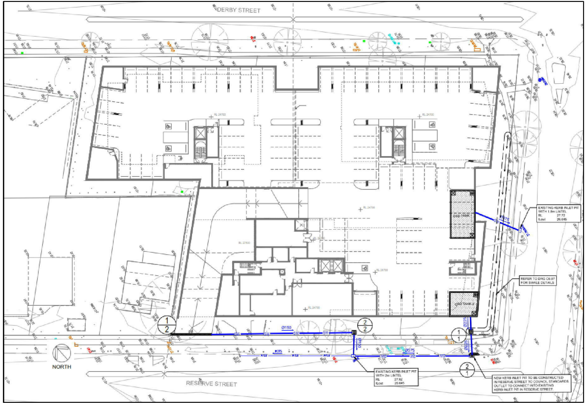
Figure 5.1: Proposed Stormwater Layout Plan
