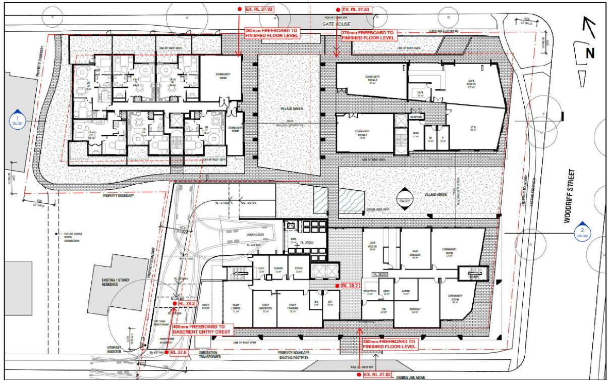
Figure 6.2: Freeboard Provided Across Development Site
