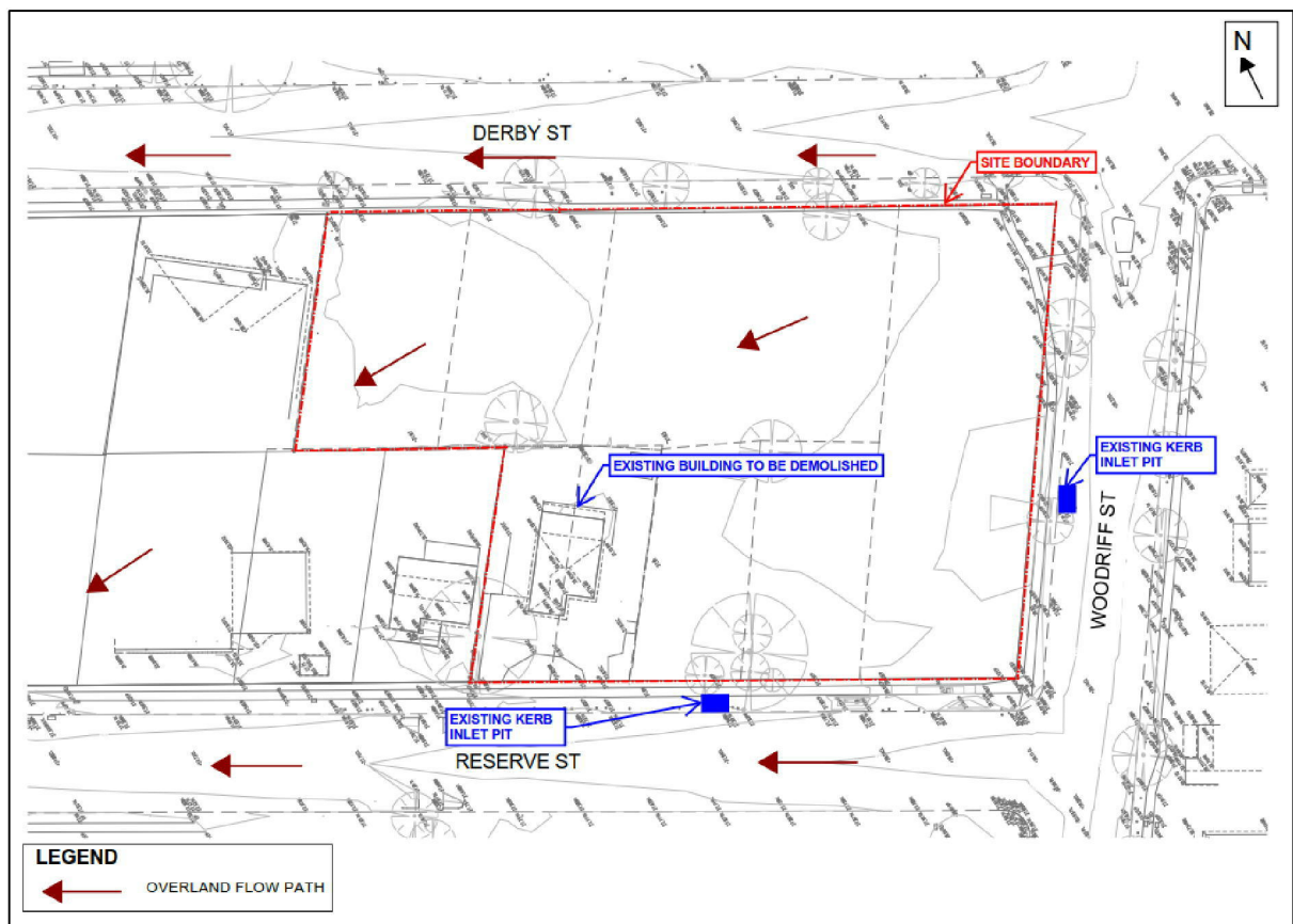
Figure 3.1: Existing Site Stormwater Network and Site Grading
