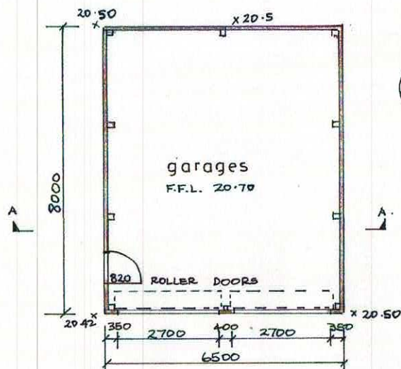
FLOOR PLAN 1:100
