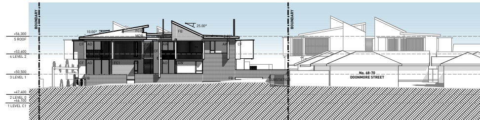
WEST ELEVATION (DOONMORE ST)
