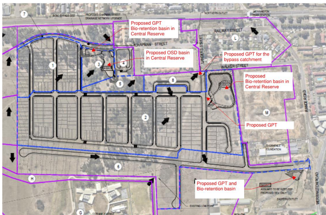
Figure 1-1 Location of stormwater infrastructure and catchments
