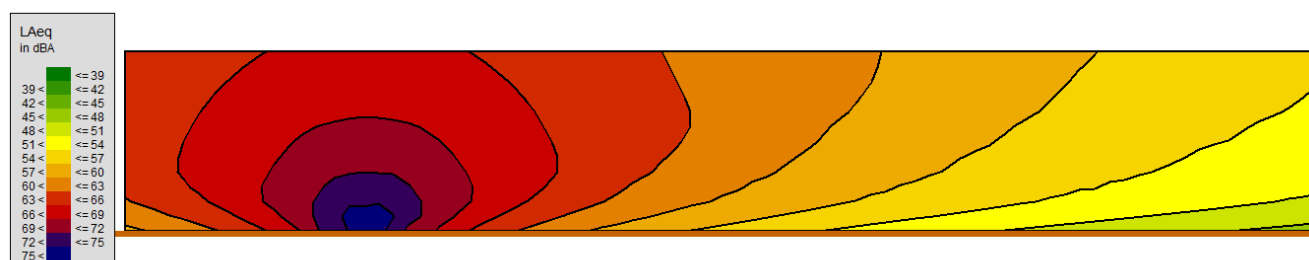
Figure 6 Cross Sectional Noise Map – Without Intervening Structures
