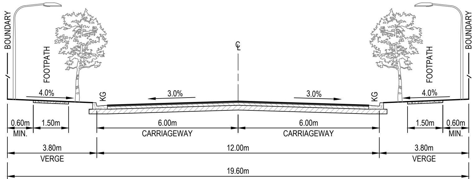
TYPICAL SECTION - NORTH SOUTH ROAD (MINOR COLLECTOR ROAD)
