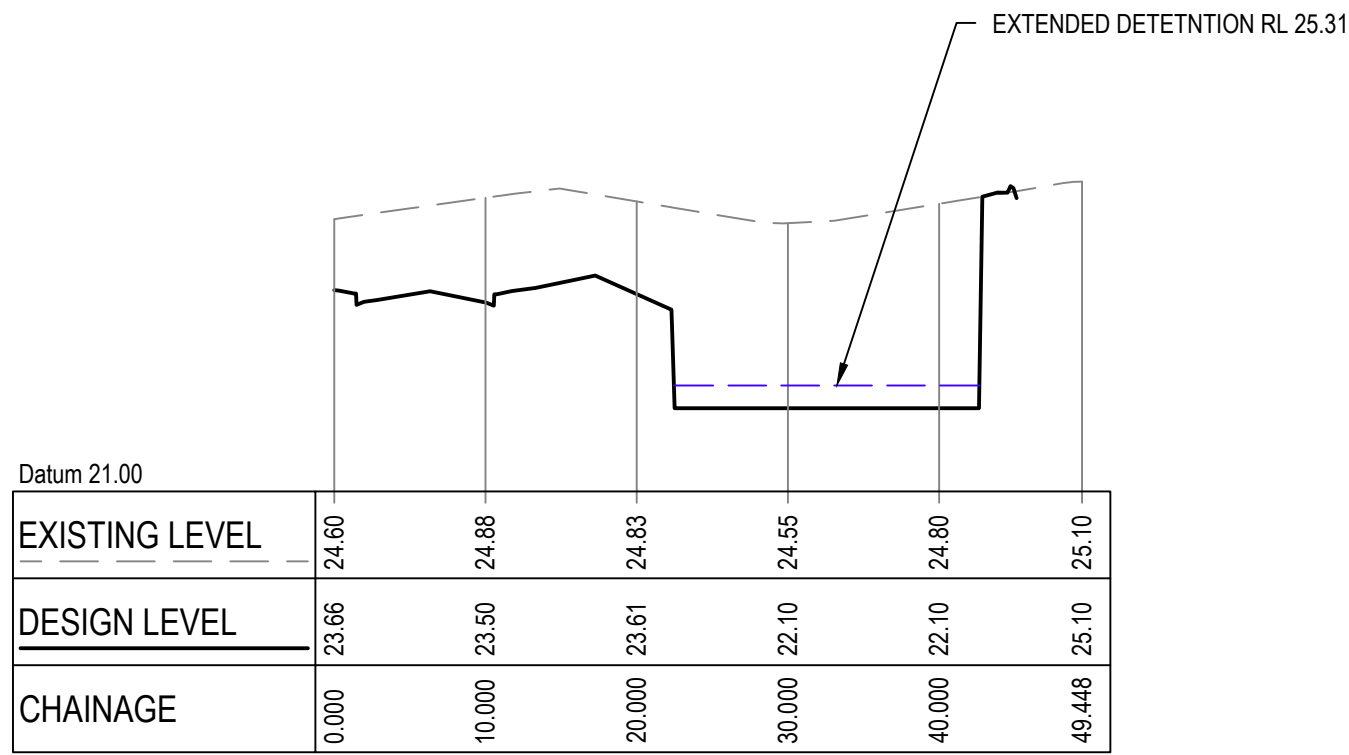
SECTION 1 SCALE 1:100V 1:500H
