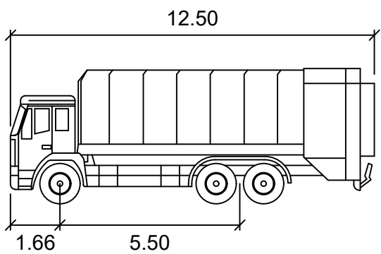
PCC 12.5 Waste Vehicle meters Width : 12.50 Track : 1.66 Lock to Lock Time : 26.1 Steering Angle : 26.1
