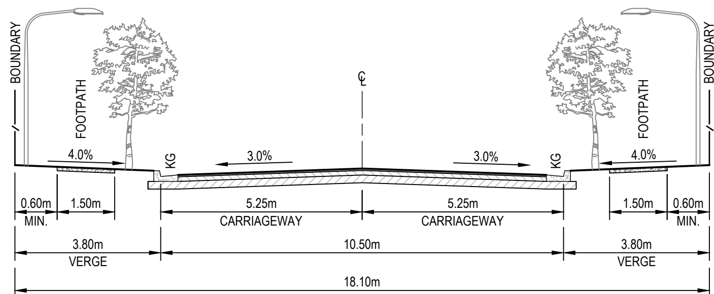
TYPICAL SECTION - LOCAL ROAD
