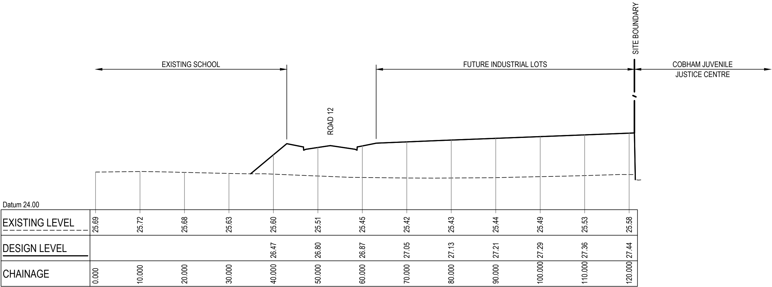
SECTION 7 SCALE 1:100V 1:500H
