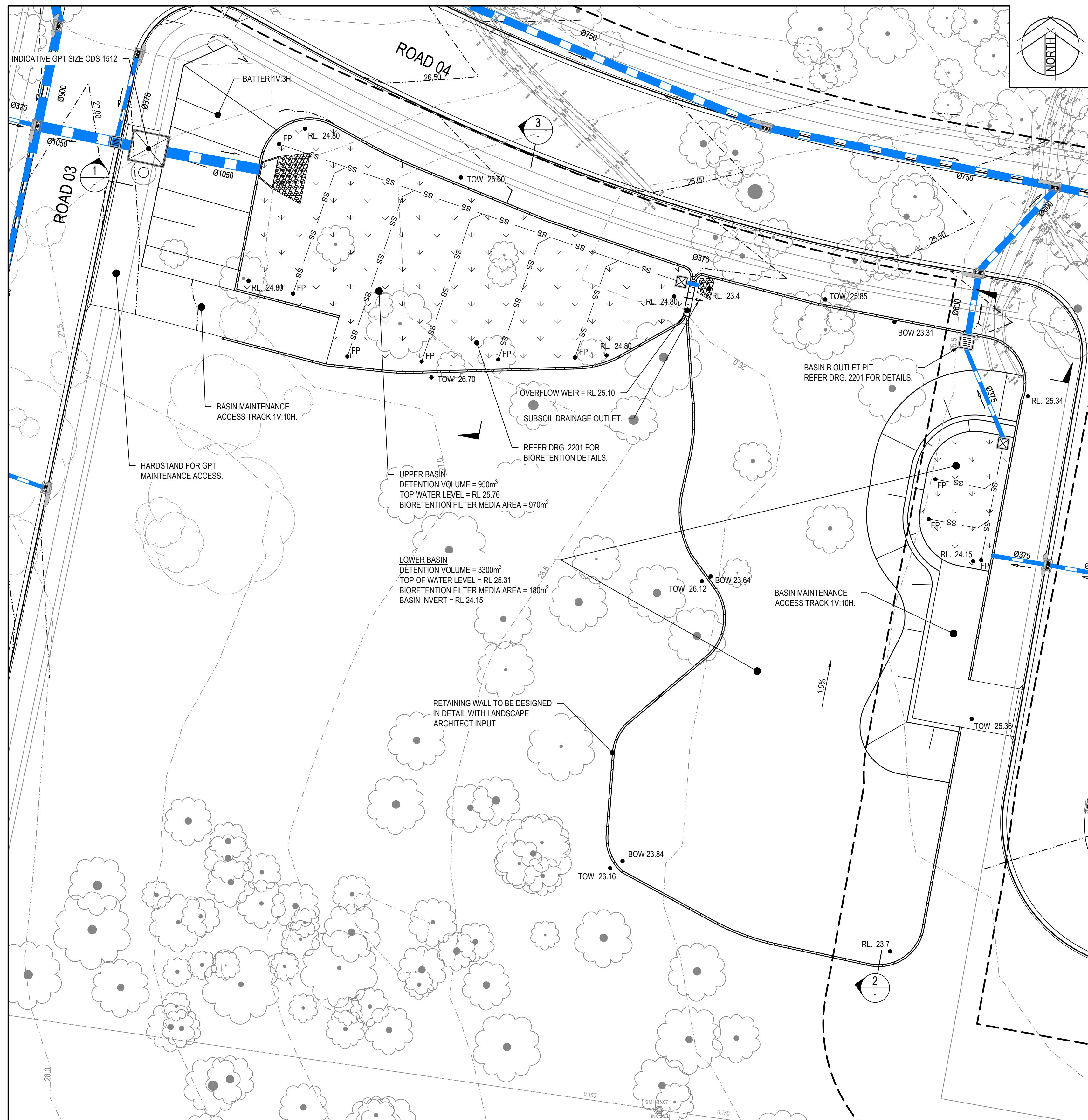
DETENTION BASIN B PLAN
