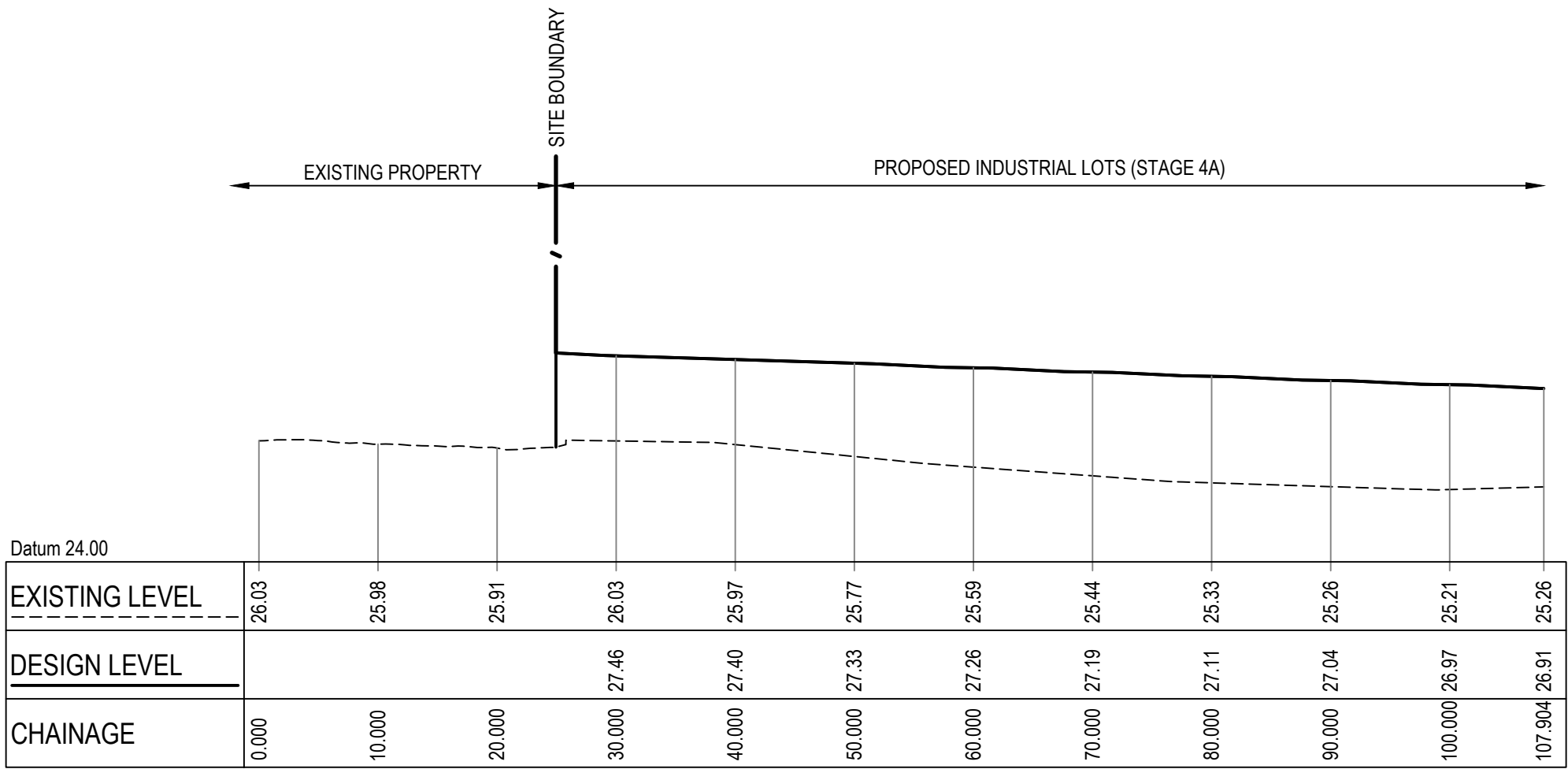
SECTION 8 SCALE 1:100V 1:500H
