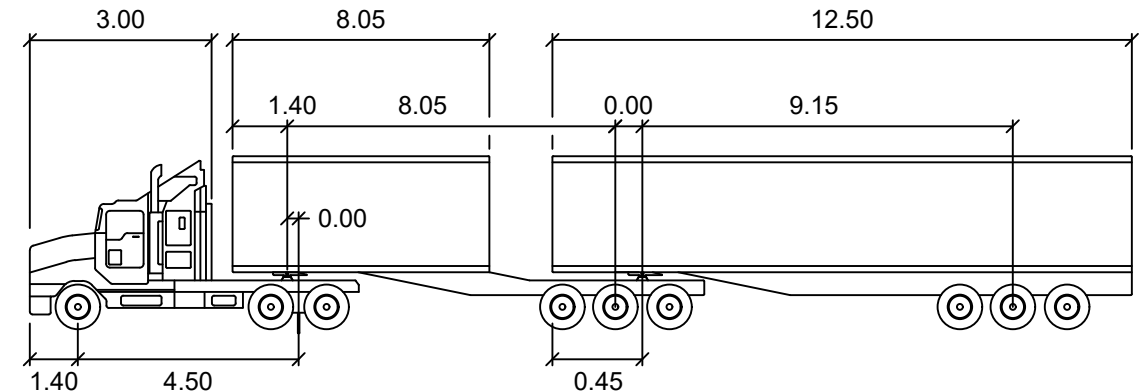
B-DOUBLE 26M
