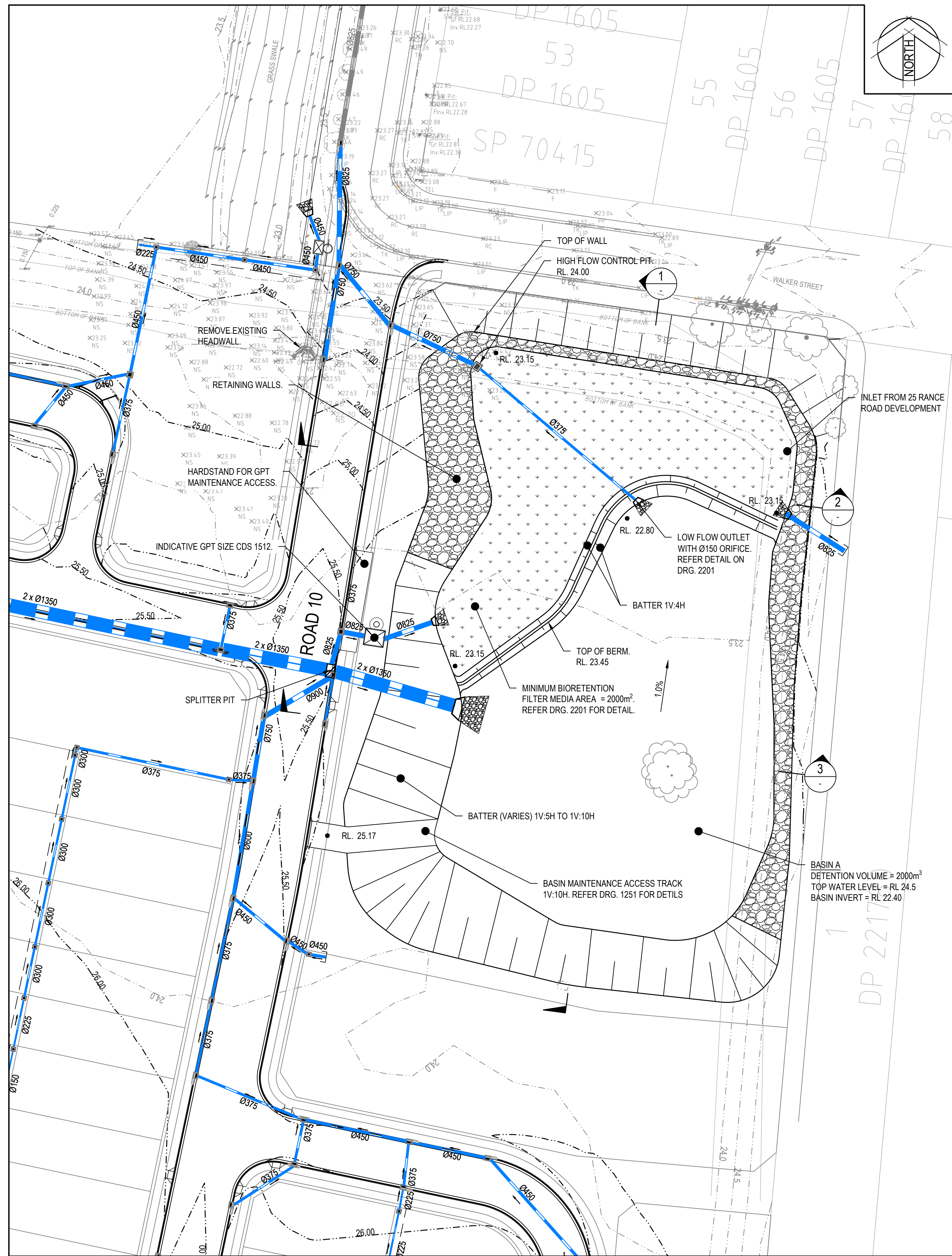
DETENTION BASIN A PLAN
