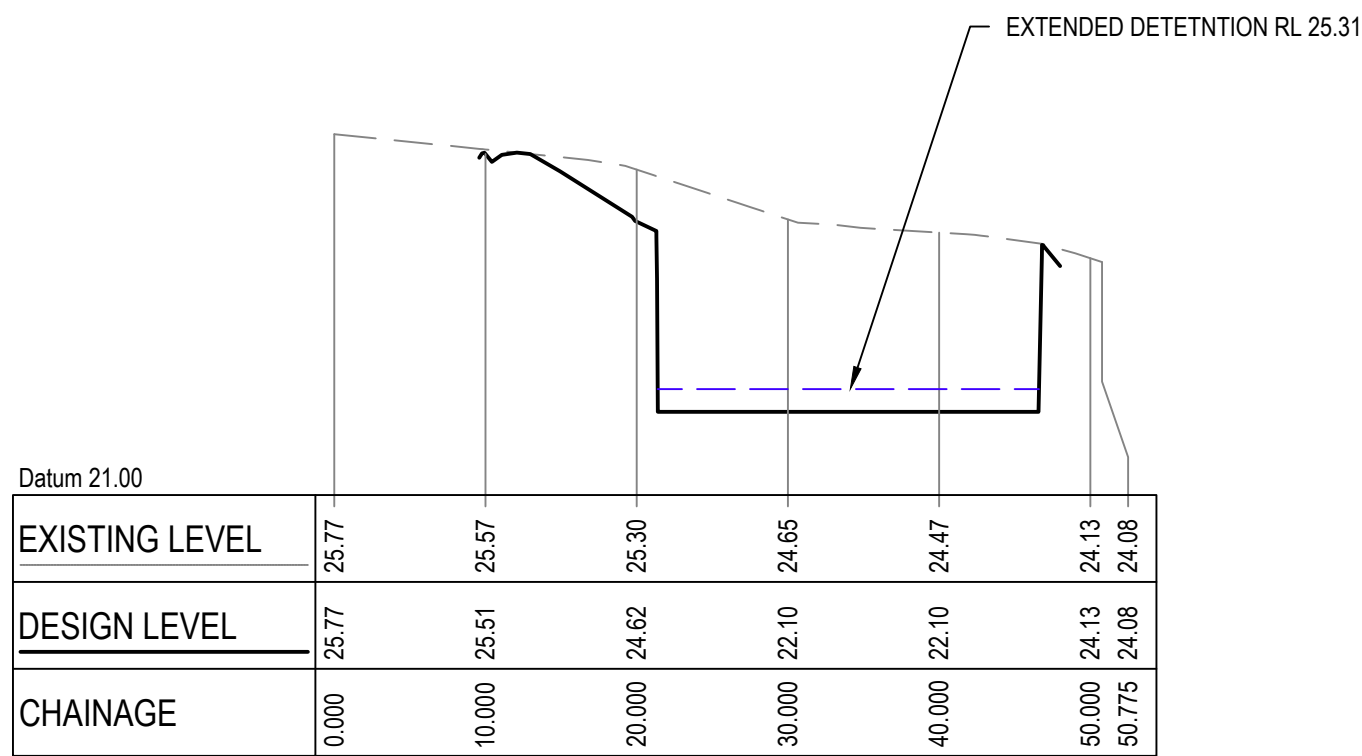
SECTION 2 SCALE 1:100V 1:500H
