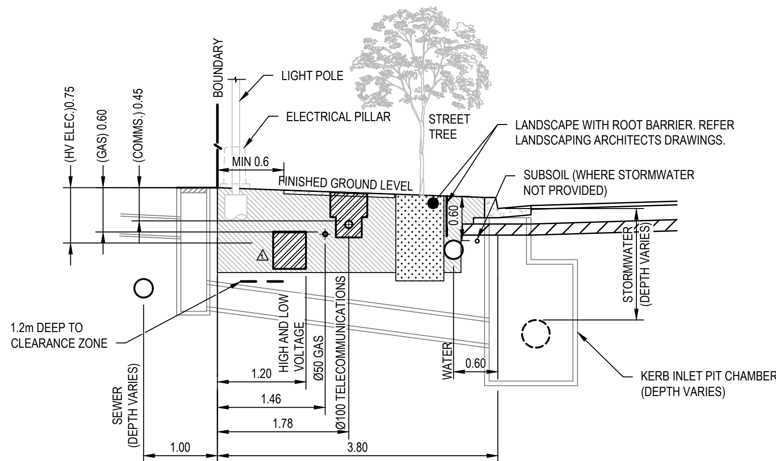
TYPICAL LOCAL ROAD SERVICES
