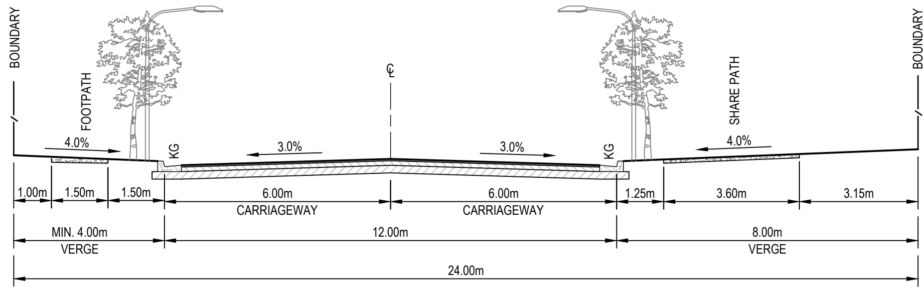
TYPICAL SECTION - EAST-WEST LINK ROAD (MAJOR COLLECTOR ROAD)
