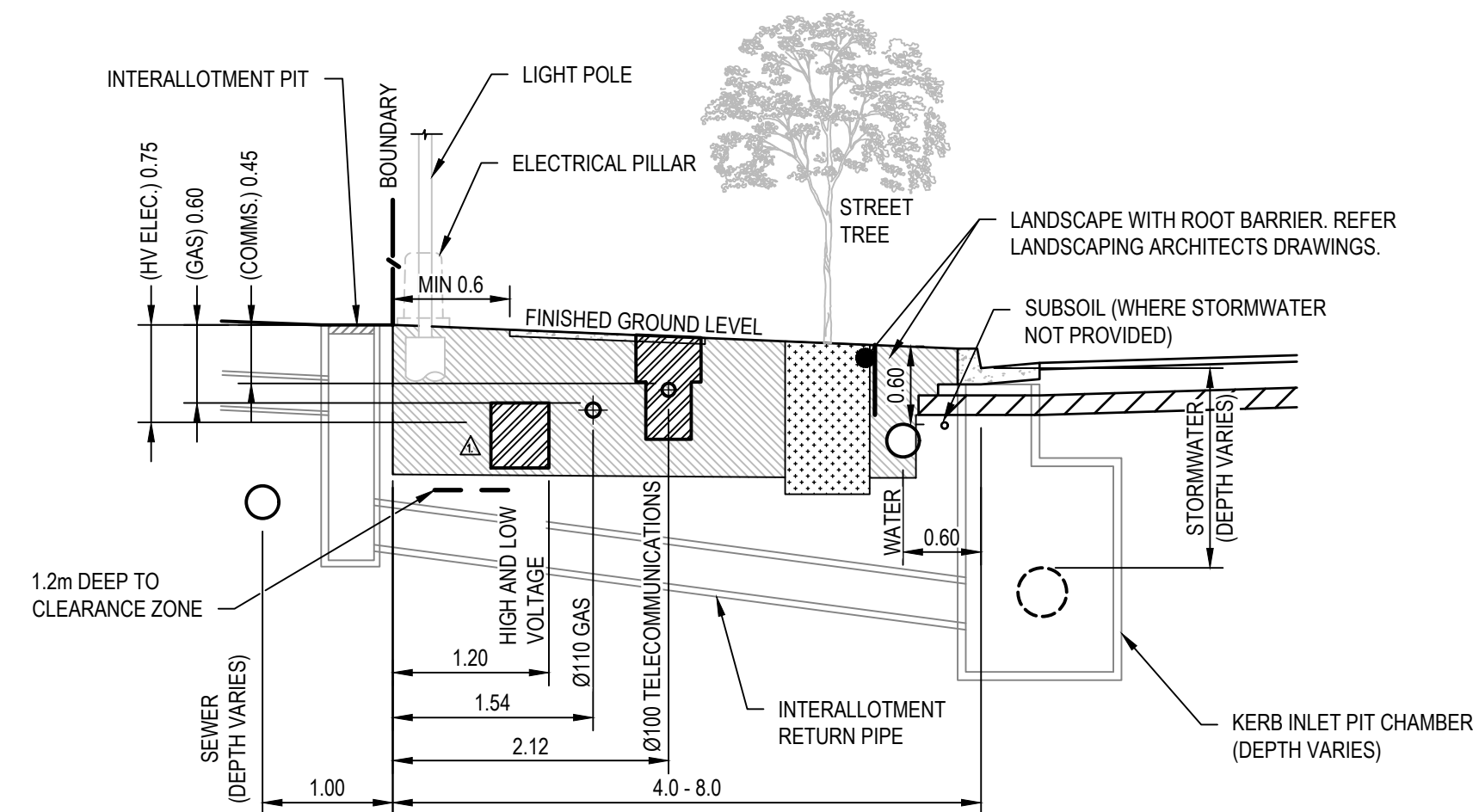
TYPICAL COLLECTOR ROAD SERVICES
