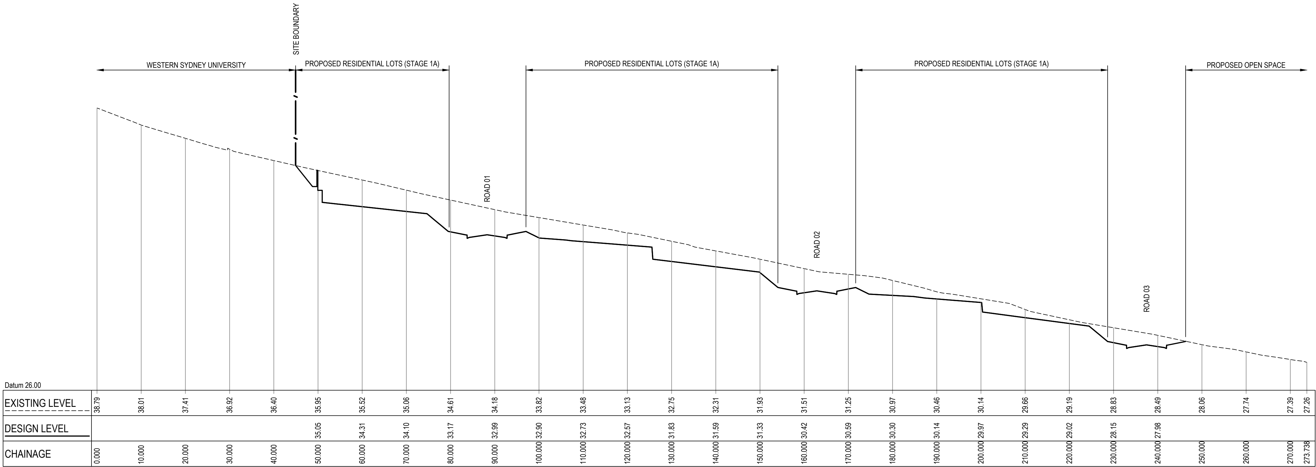
SECTION 12 SCALE 1:100V 1:500H
