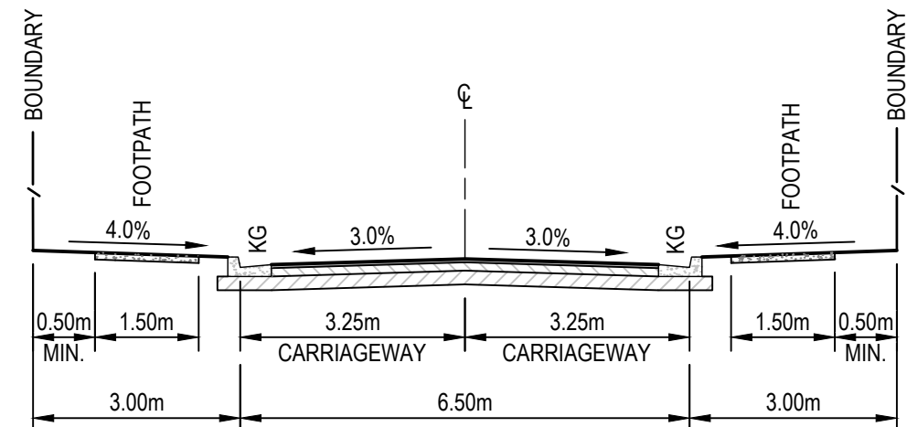
TYPICAL SECTION - LANEWAY
