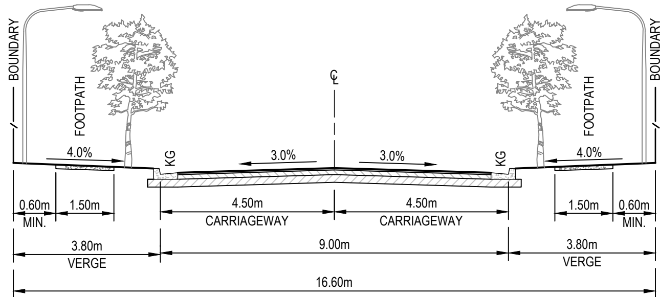
TYPICAL SECTION - MINOR LOCAL ROAD
