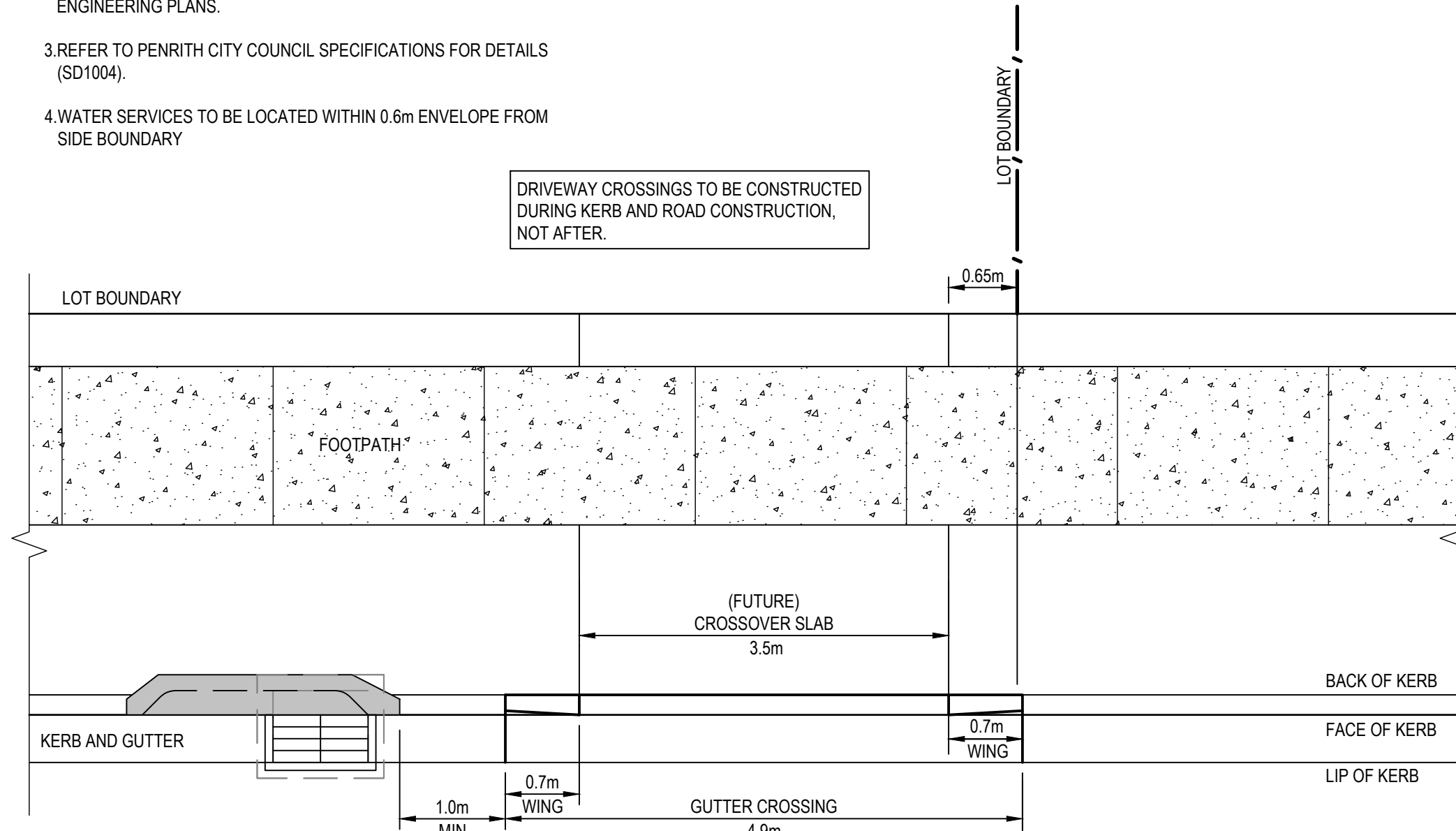
TYPICAL DRIVEWAY LOCATION DETAIL
