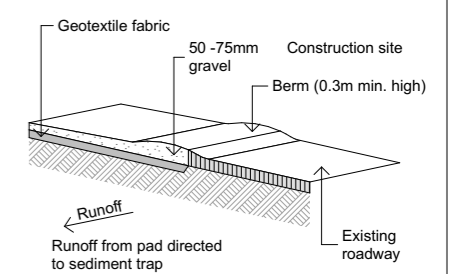
TEMPORARY CONSTRUCTION EXIT
