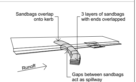
SANDBAG KERB INLET SEDIMENTATION TRAP
