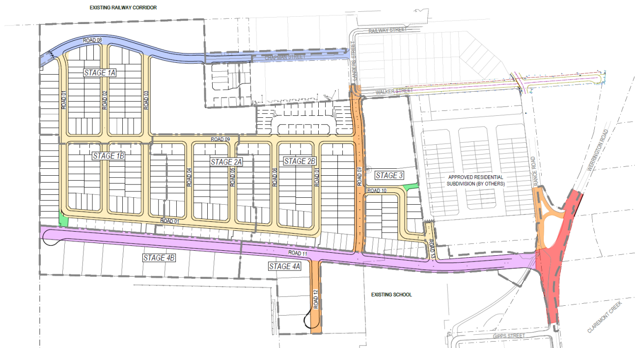
Figure 3-1 Road Hierarchy Plan (Drawing CI 1041)
