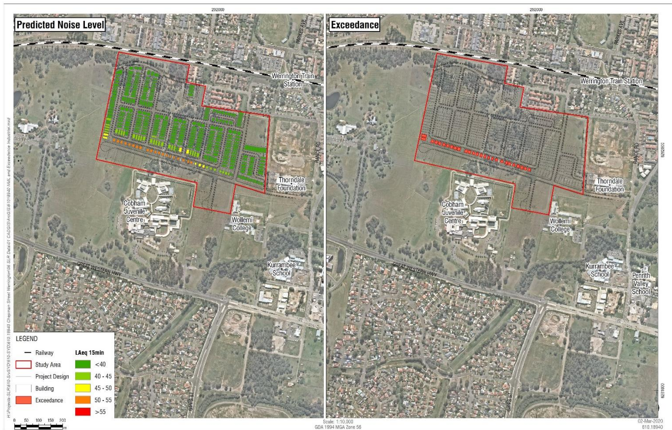
Figure 5 Industrial Noise Impacts – Daytime
