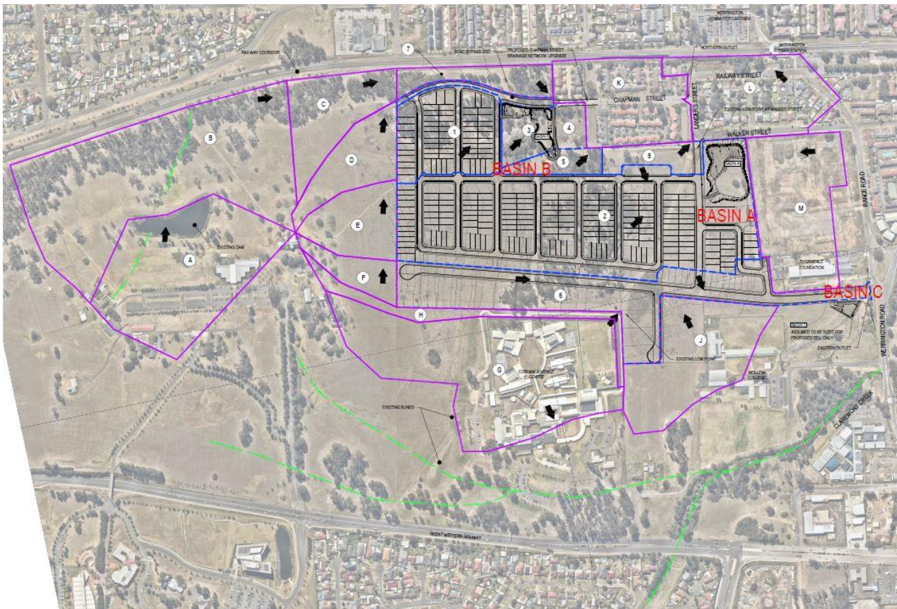
Figure 6-2 Post Development Catchment Plan
