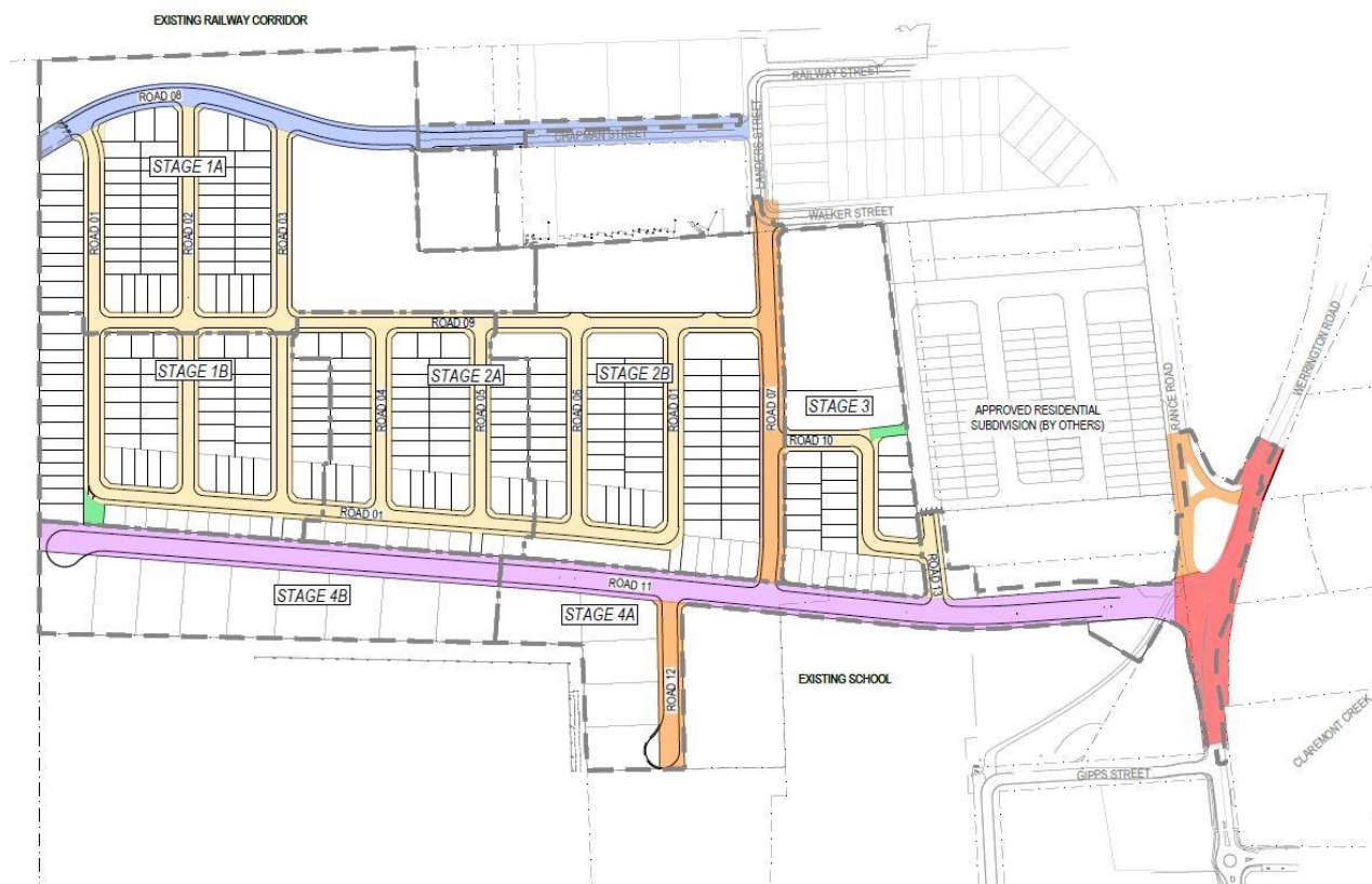
Figure 3-1 Road Hierarchy Plan (Drawing CI 1041)
