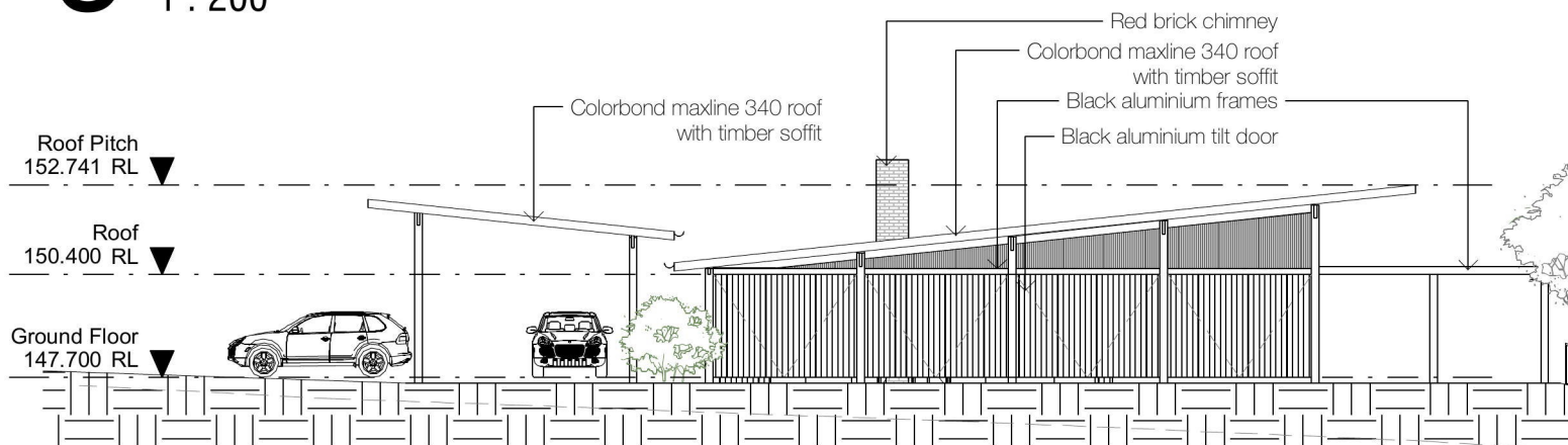
5 Notification - South West (End) 1 : 200
