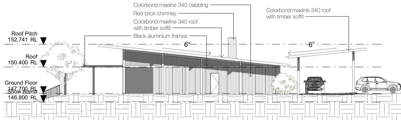
3 Notification - North East (End) 1 : 200
