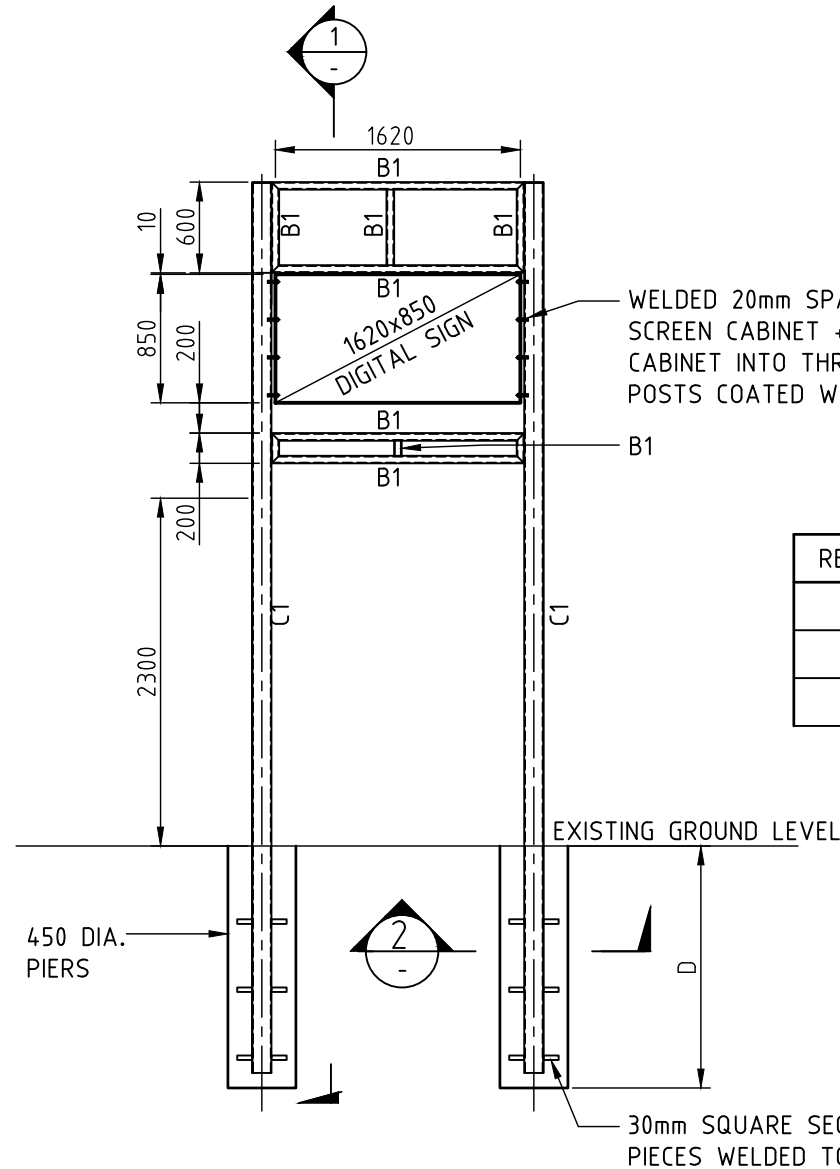
ELEVATION A SCALE 1:50
