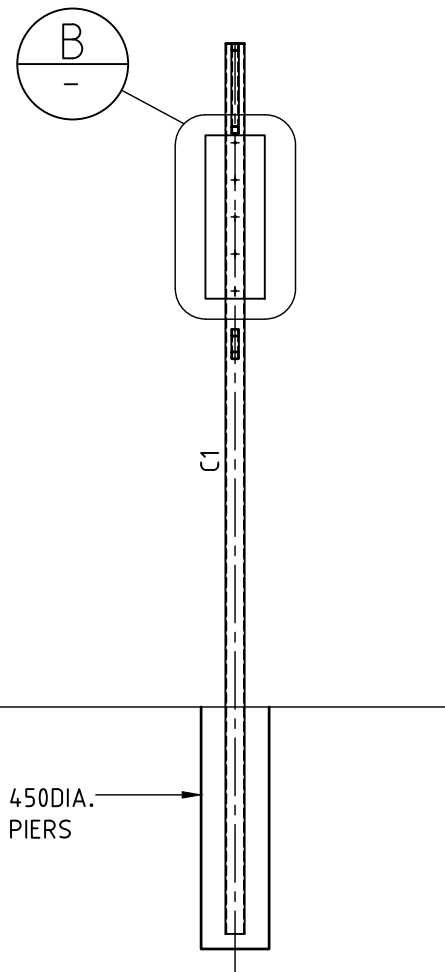
SECTION 1 SCALE 1:50
