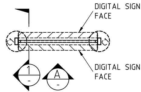
PLAN SCALE 1:50
